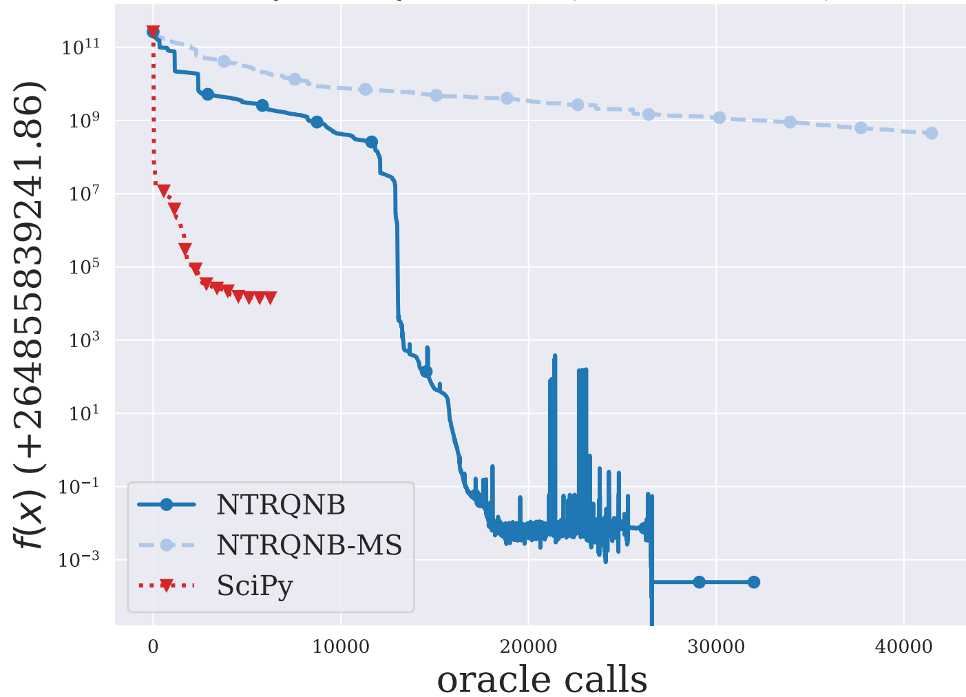
QRTQUAD ( n = 5000 )
