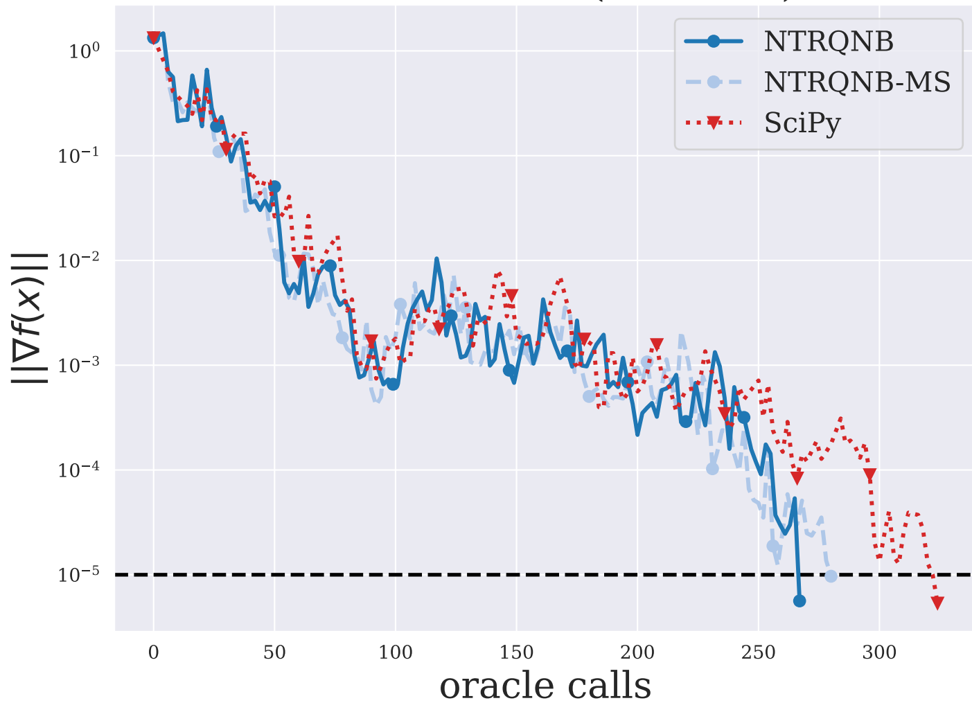
SANTALS ( n = 21 )
