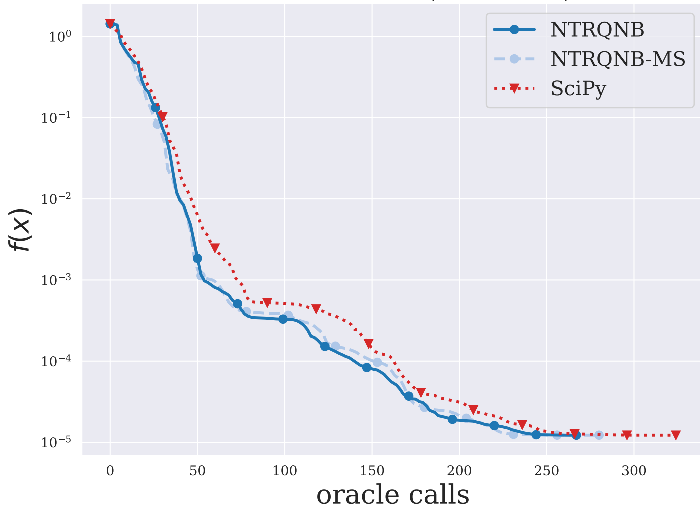
SANTALS ( n = 21 )
