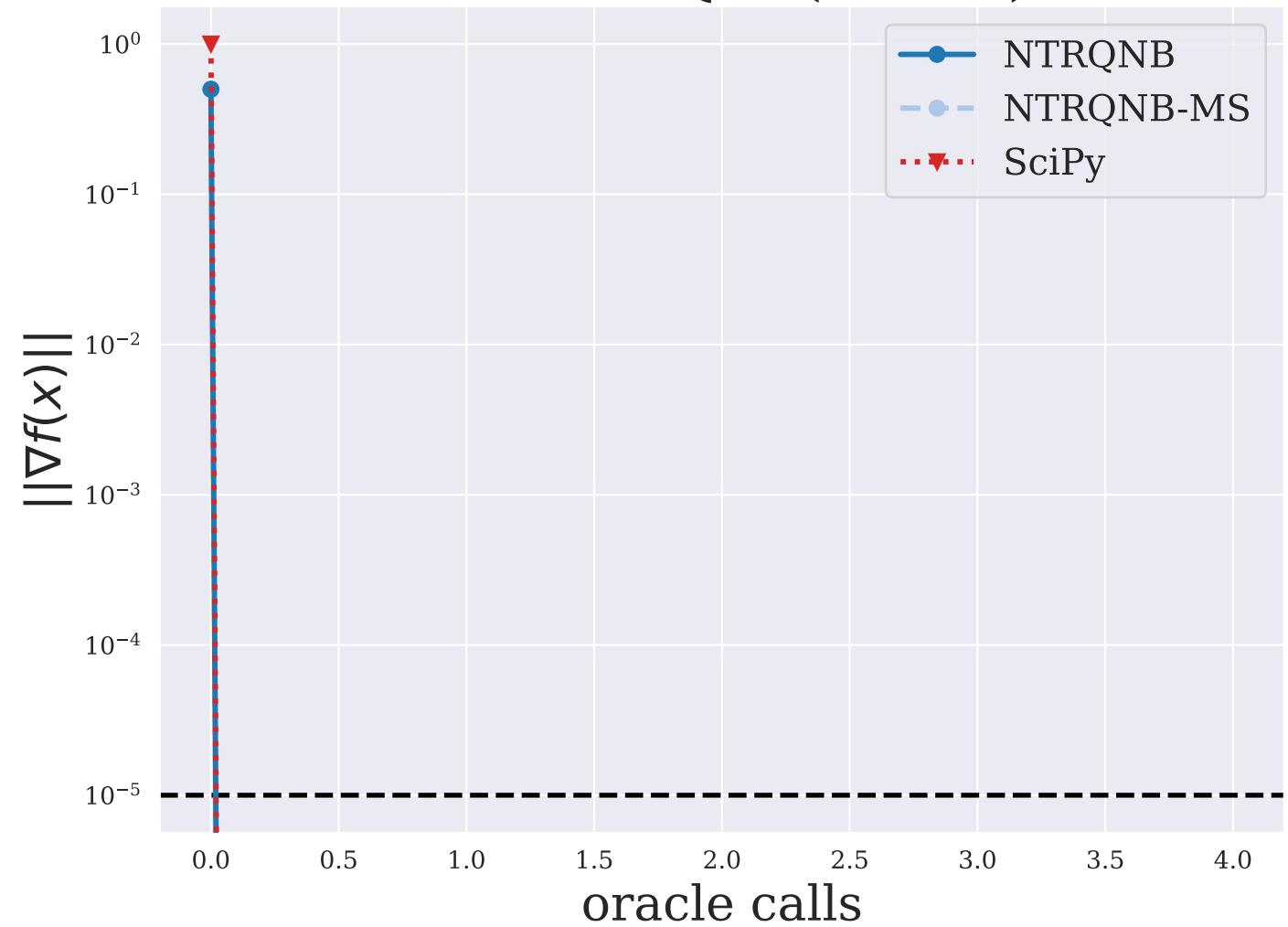
SIM2BQP ( n = 1 )
