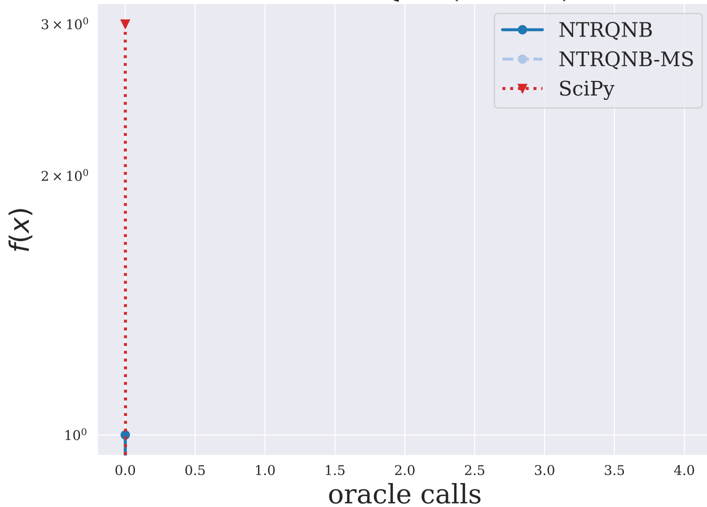
SIM2BQP ( n = 1 )
