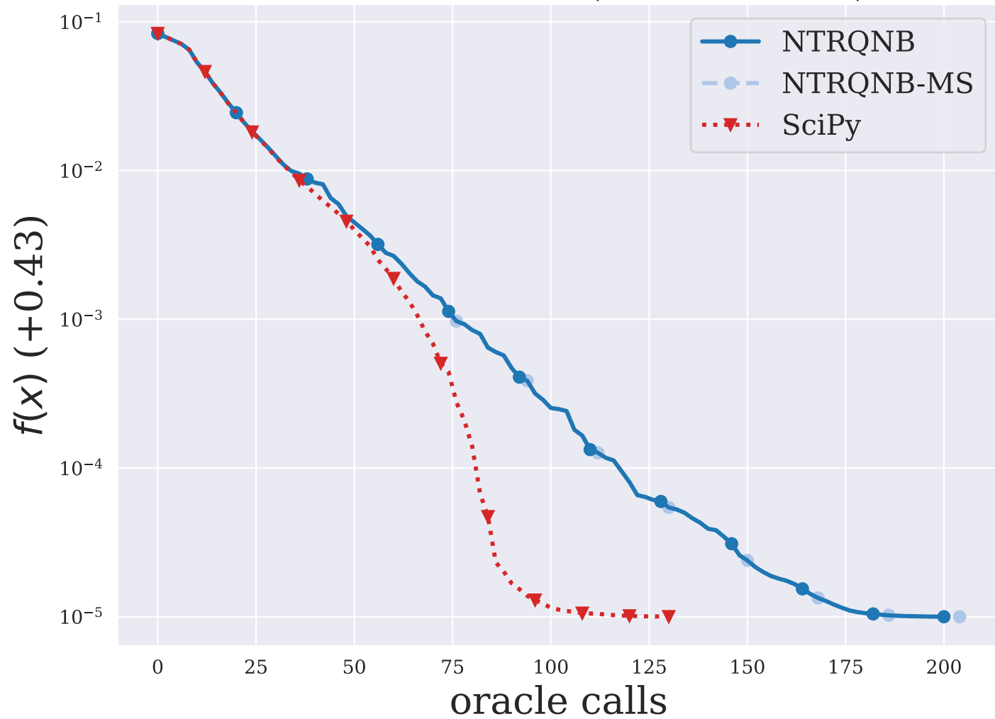
TORSION1 ( n = 5184 )
