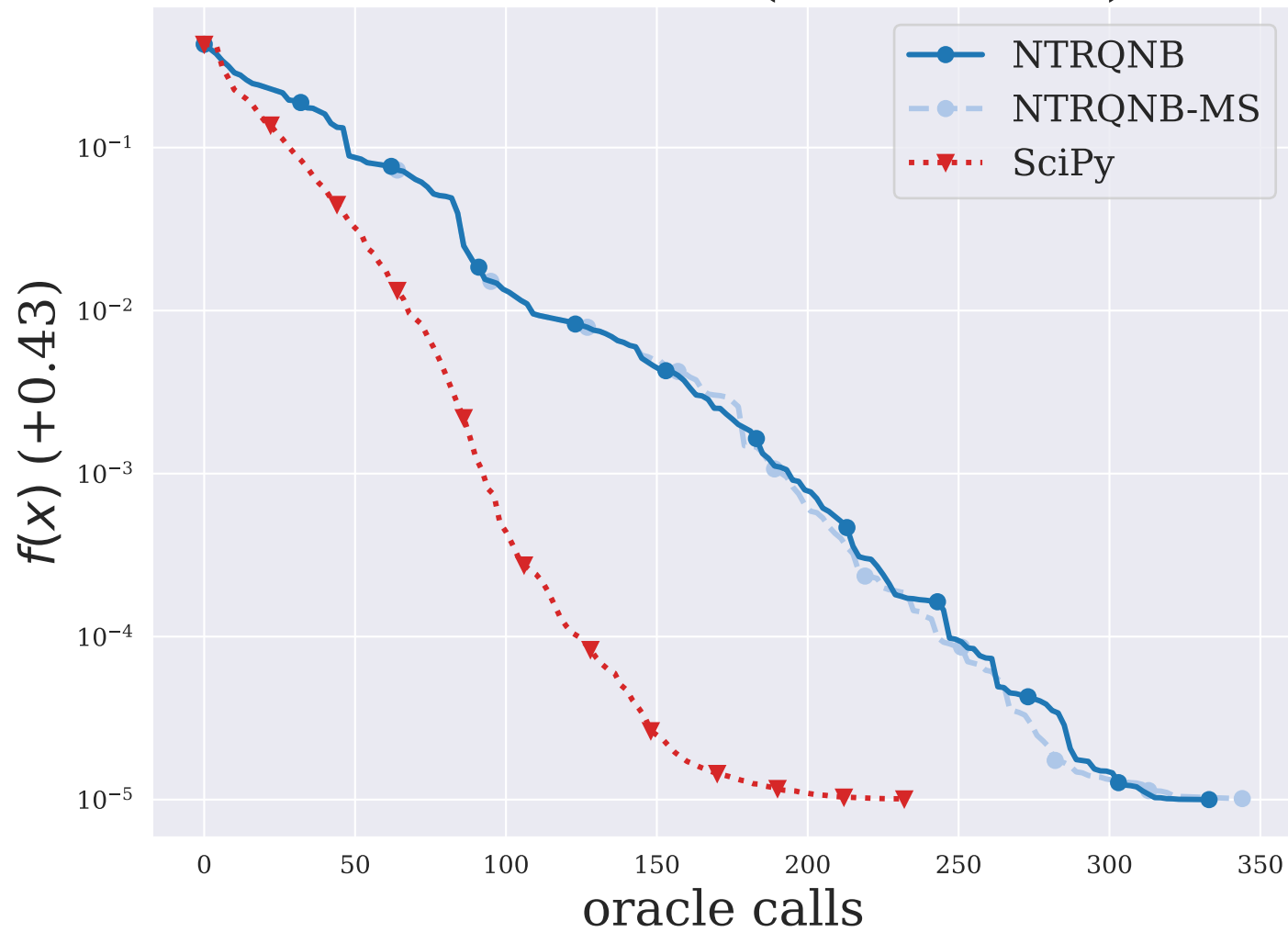
TORSION2 ( n = 5184 )
