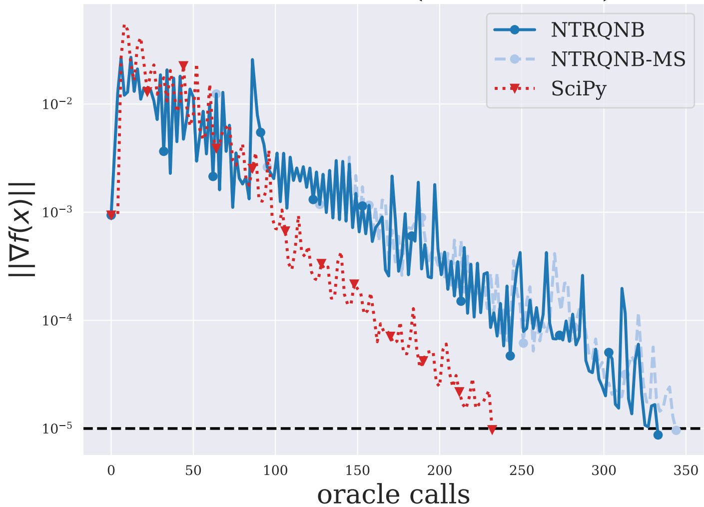
TORSION2 ( n = 5184 )
