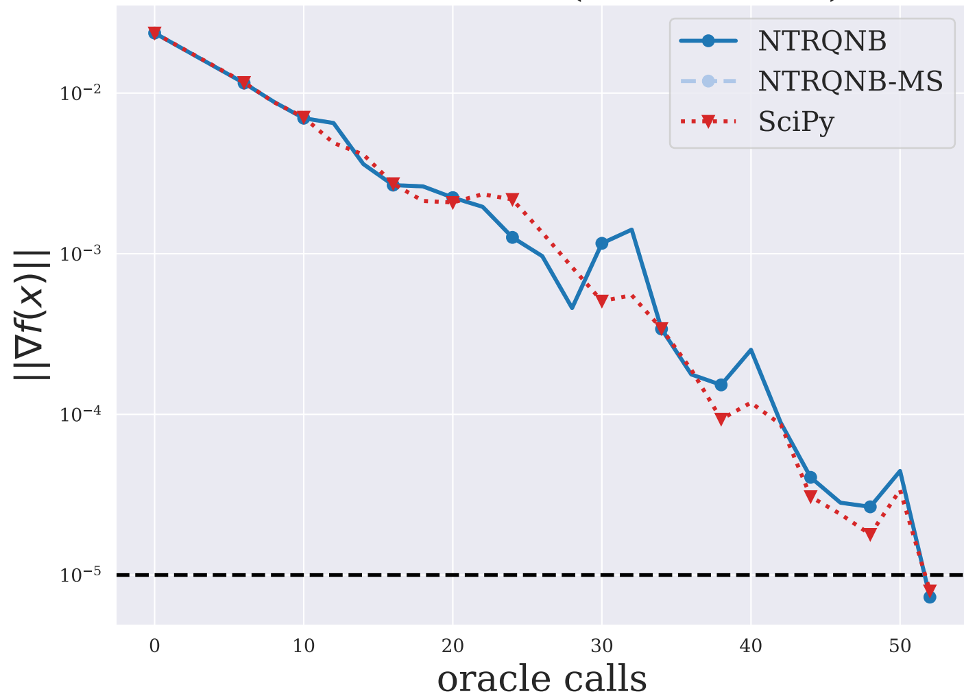
TORSION5 ( n = 5184 )
