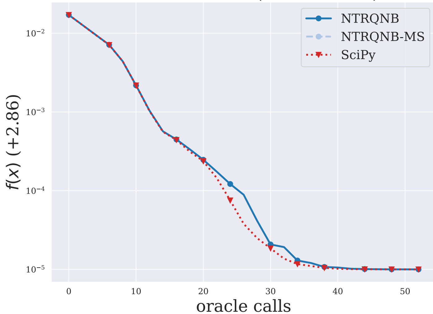
TORSION5 ( n = 5184 )
