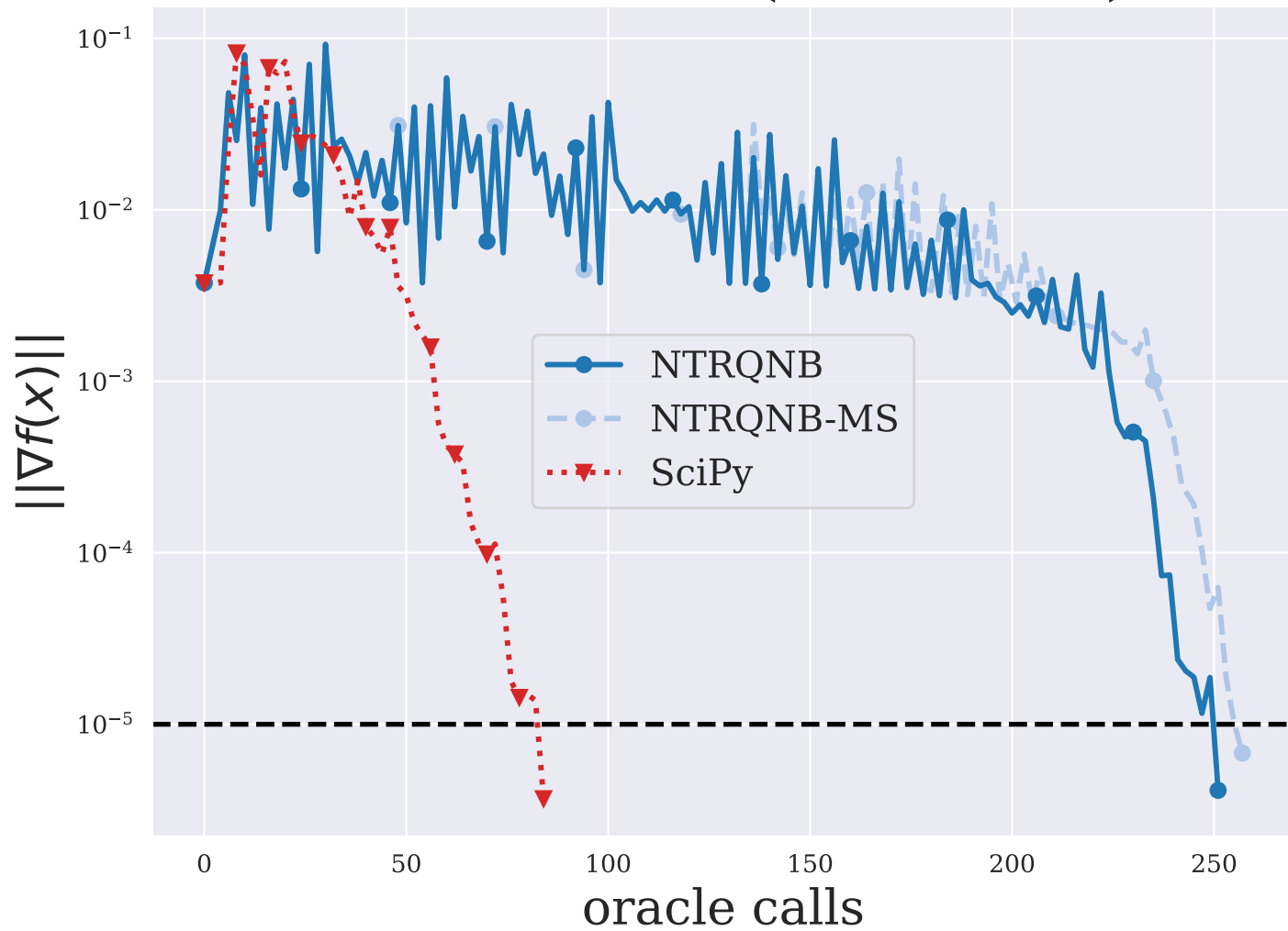
TORSION6 ( n = 5184 )
