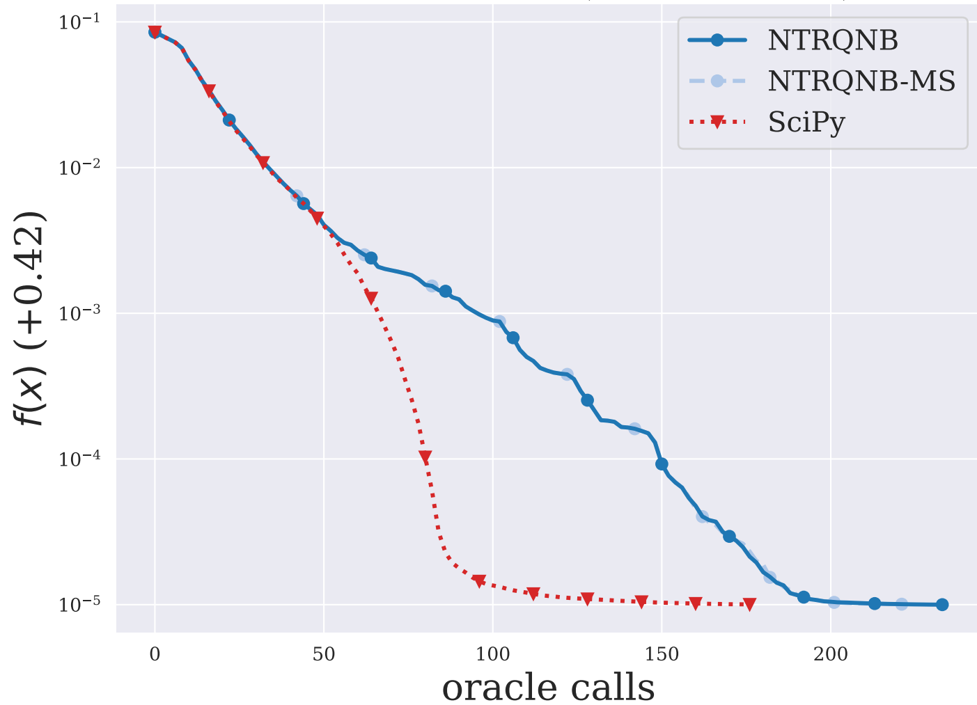
TORSIONA ( n = 5184 )
