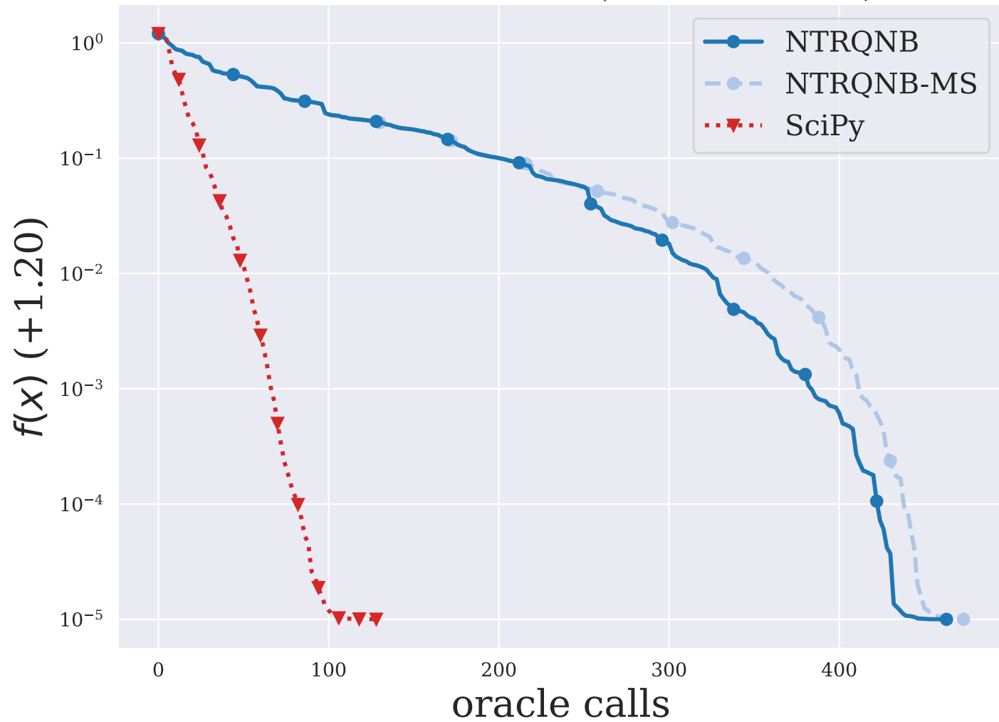
TORSIOND ( n = 5184 )
