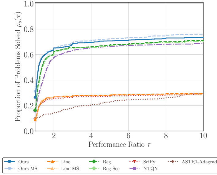
Fig. 2: Performance profile for the deliberately adverse joint function-and-gradient noise setting (componentwise level 10^{-3} ) and \epsilon_{\text{gtol}} = 10^{-2} . This experiment lies outside the exact-gradient theory.
