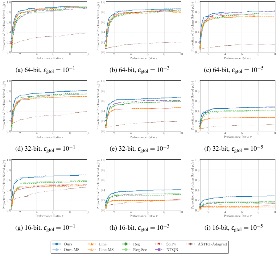
Fig. 4: Performance profiles across floating-point precisions (64-, 32-, and 16-bit) and tolerance levels.
