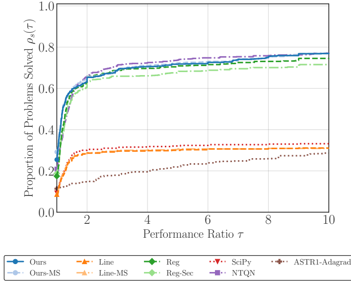
Fig. 1: Theory-aligned function-value-noise results at noise level 10^{-3} , supplied error bound \varepsilon_f = 10^{-2} , and \varepsilon_{\text{gtol}} = 10^{-2} .
