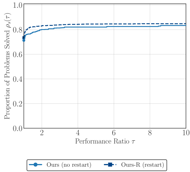
Fig. 6: Performance profile for the restart ablation on the same 1,100 paired function-noise instances as the primary experiment. Ours is the analyzed method with no accumulator restart. Ours-R applies the optional rule in eq. (37) with at most ten restarts. The close curves agree with the paired call counts: restart changes aggregate success only slightly and is not uniformly faster.
