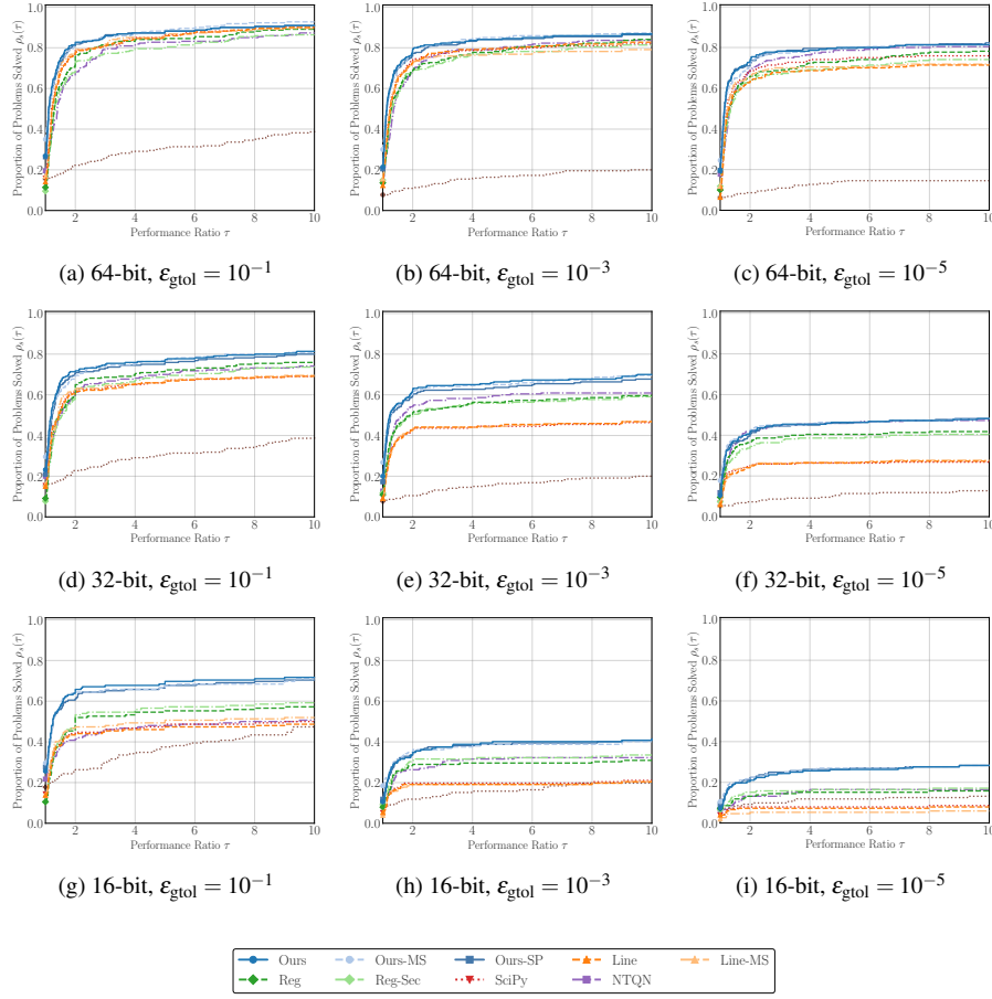
Fig. 2: Performance profiles across different floating-point precisions (64-, 32-, and 16-bit) and tolerance levels. The results demonstrate the robustness of the proposed methods.
