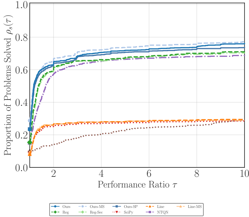
Fig. 1: Performance profile for artificial noise setting (level of 10^{-3} ) and \epsilon_{\text{gtol}} = 10^{-2} .
