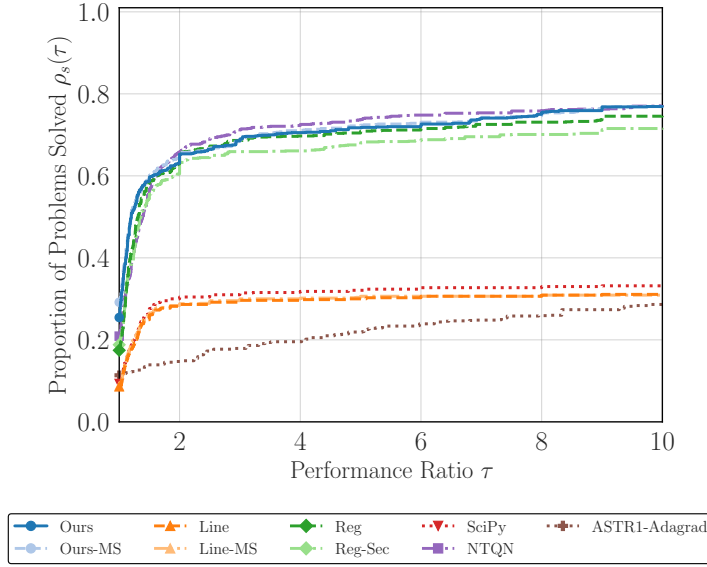
Fig. 1: Theory-aligned function-value-noise results at noise level 10^{-3} , supplied error bound \epsilon_f = 10^{-2} , and \epsilon_{\text{gtol}} = 10^{-2} .
