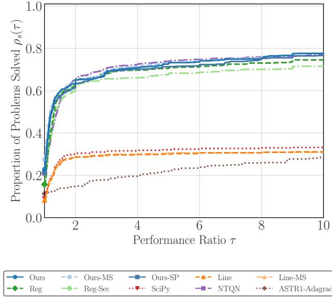
Fig. 1: Theory-aligned function-value-noise results at noise level 10^{-3} , supplied error bound \epsilon_f = 10^{-2} , and \epsilon_{\text{gtol}} = 10^{-2} .
