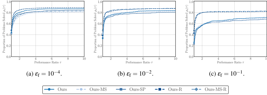
Fig. 3: Performance profiles for error-bound misspecification under function-value-only noise of level 10^{-3} and \varepsilon_{\text{gtol}} = 10^{-2} .
