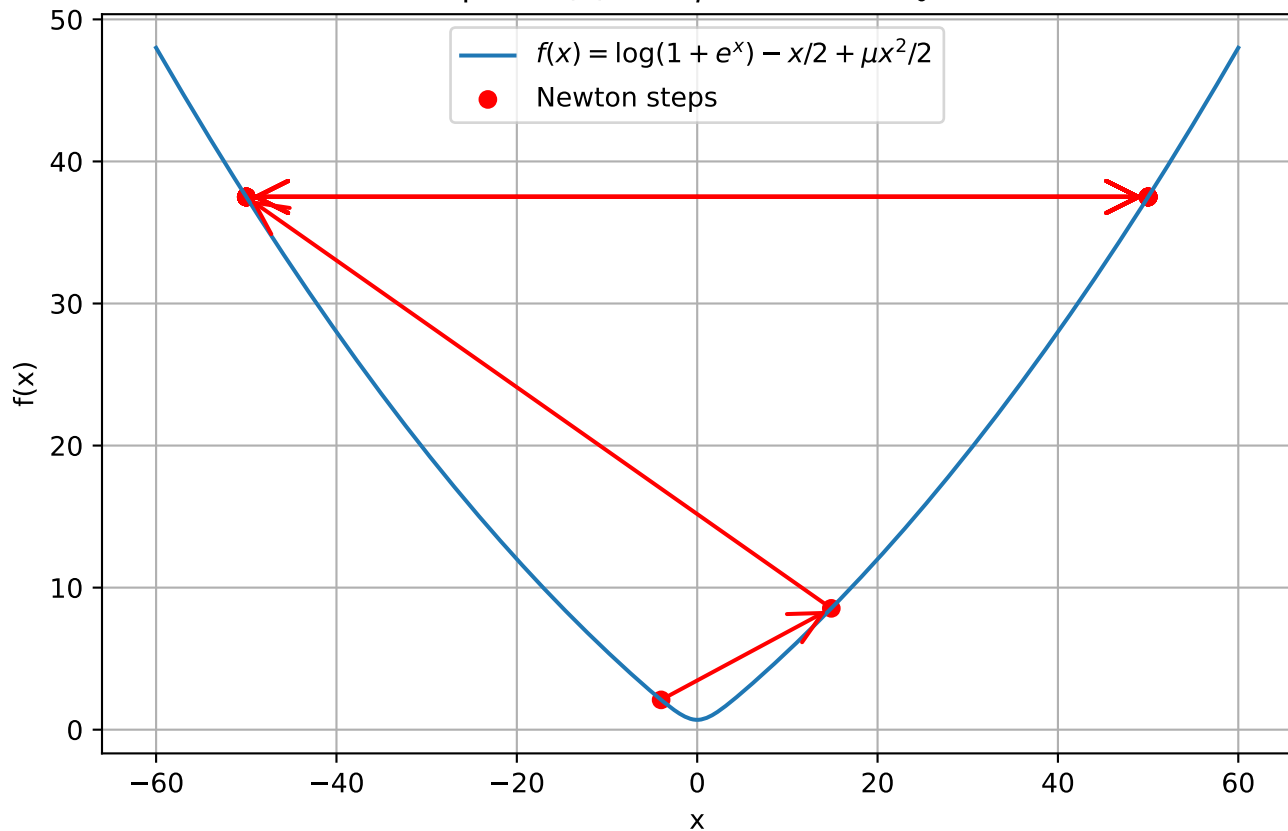
Graph of f(x) with \mu=0.01 and x_0=-4
