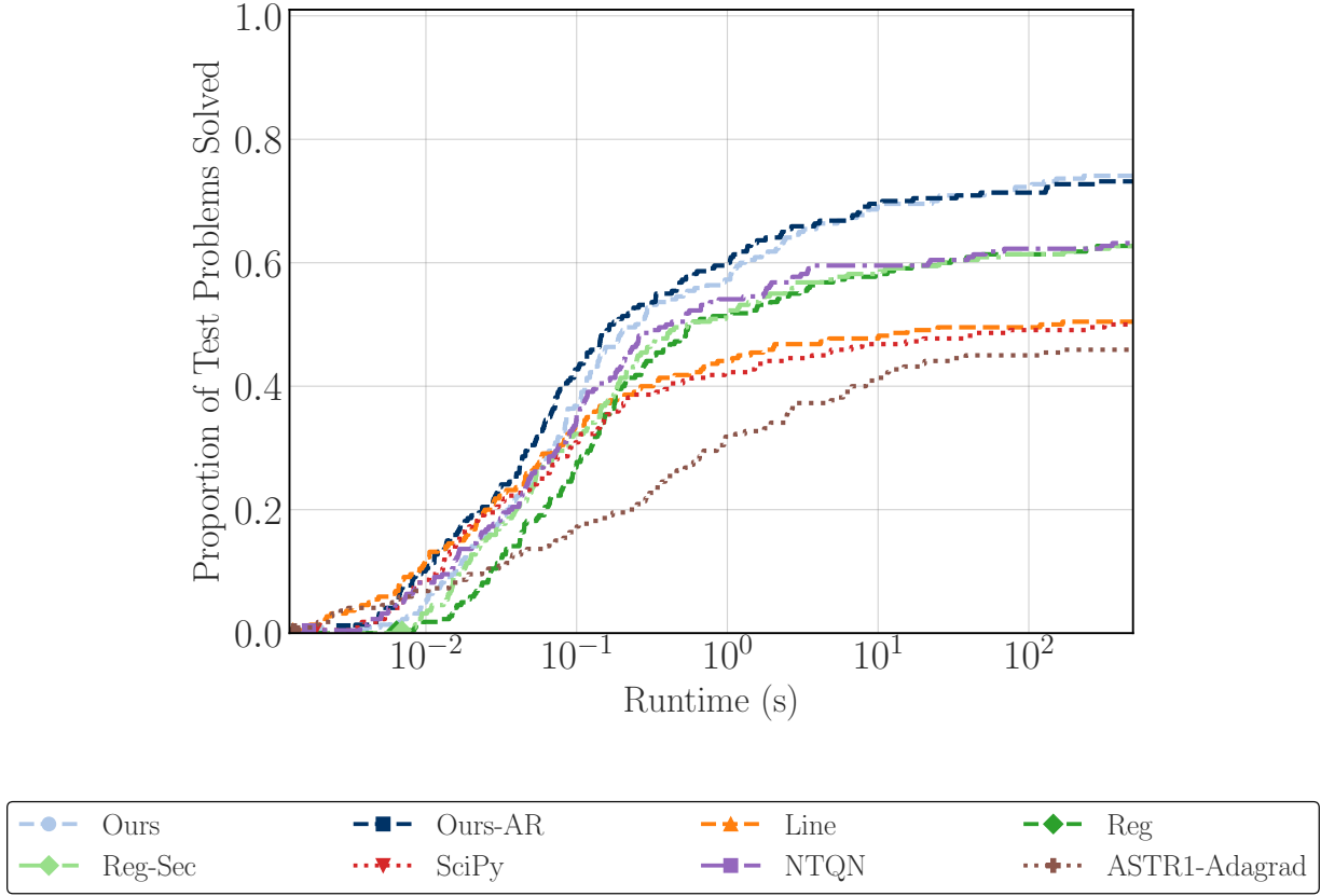
Figure 6: Time-to-solution comparison with 32-bit evaluations and \epsilon_{\text{gtol}} = 10^{-3} . Each curve shows the fraction of problems reaching the gradient tolerance within the elapsed time.
