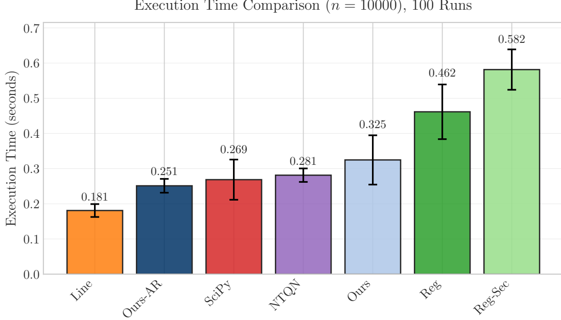
Figure 5: Mean execution time for 100 iterations on the ill-conditioned quadratic problem. Error bars show one standard deviation over 100 runs.
