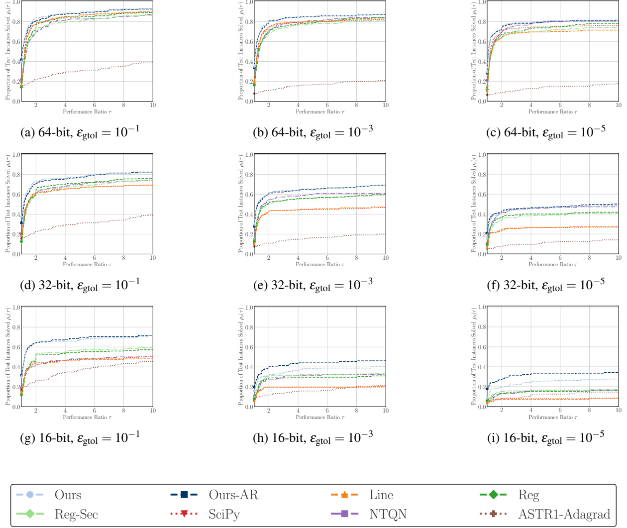
Figure 4: Performance profiles across evaluation precisions and gradient tolerances.
