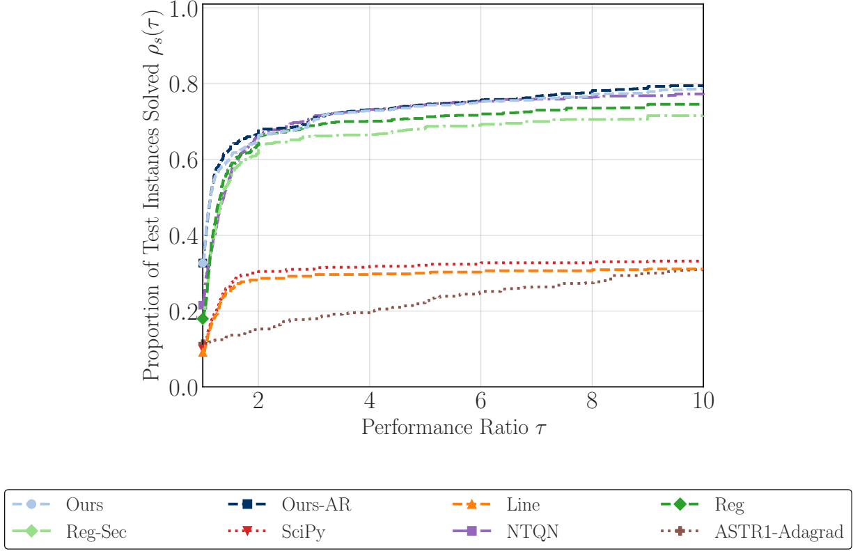
Figure 1: Performance profiles under function-value noise of level 10^{-3} , with exact gradients, \epsilon_f = 10^{-2} , and \epsilon_{\text{gtol}} = 10^{-2} .
