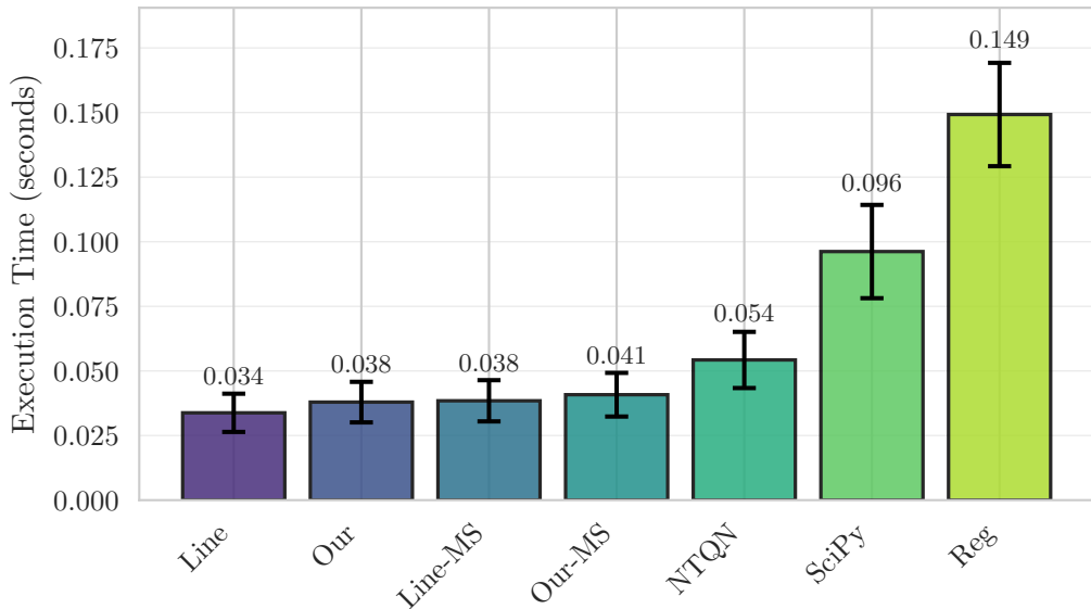
Execution Time Comparison ( n = 10000 ), 100 Runs
