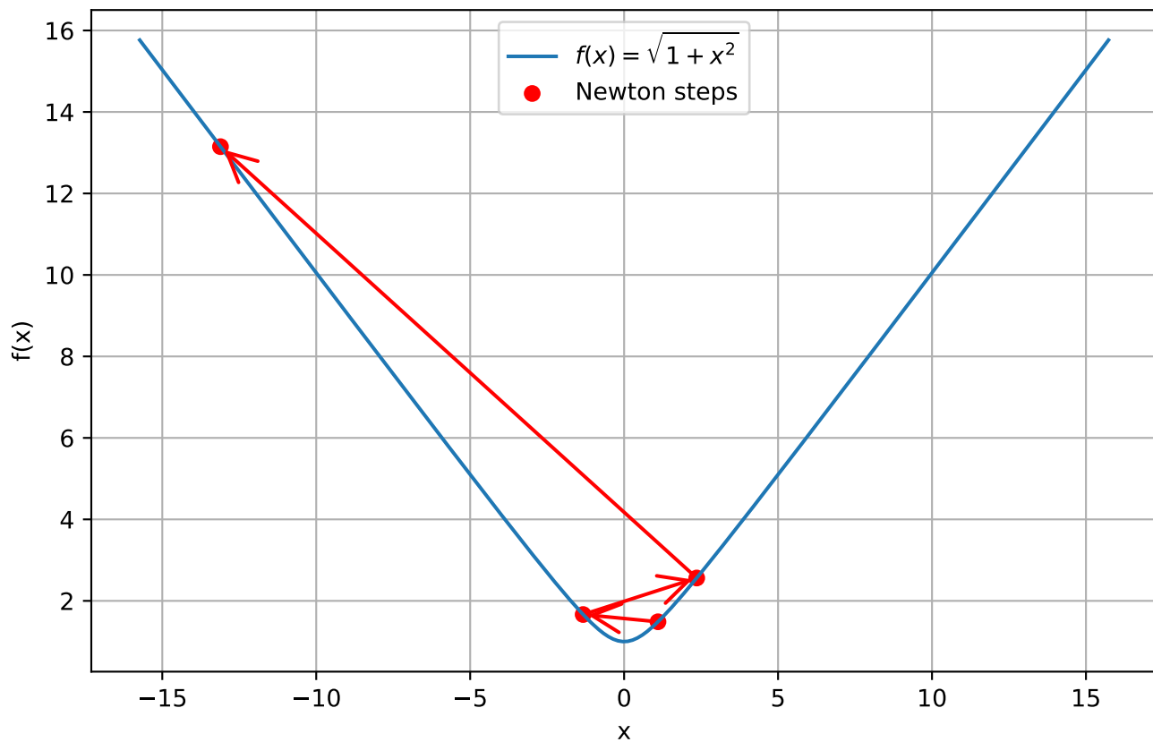
Graph of f(x) with x_0=1.1
