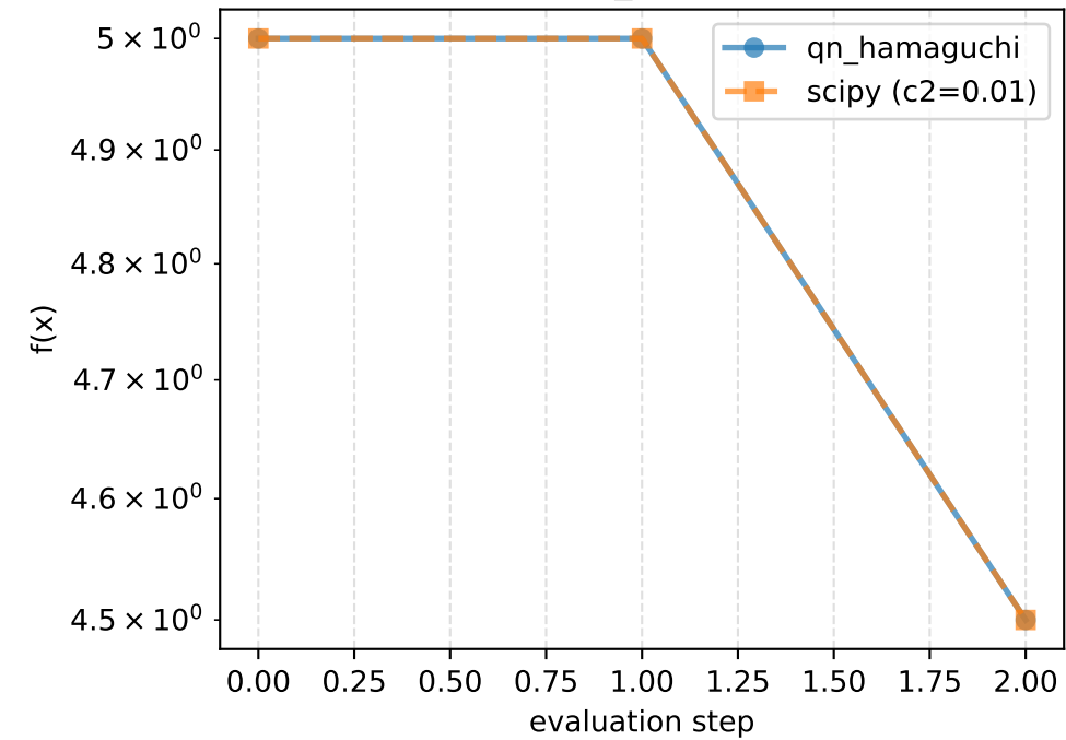
ConvexEvenPolynomial_2 - Function value history
