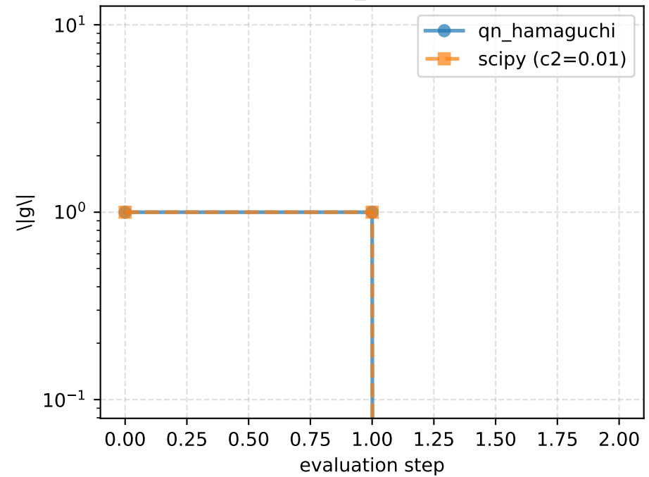
ConvexEvenPolynomial_2 - Gradient norm history
