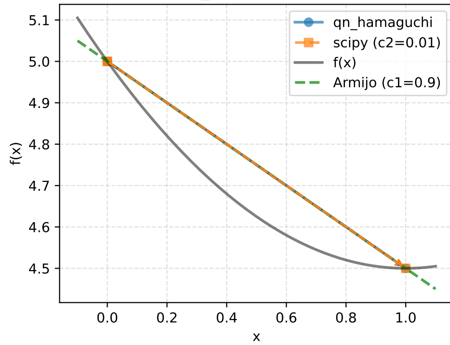
ConvexEvenPolynomial_2 - Function value and search paths
