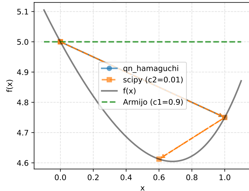
ConvexEvenPolynomial_4 - Function value and search paths
