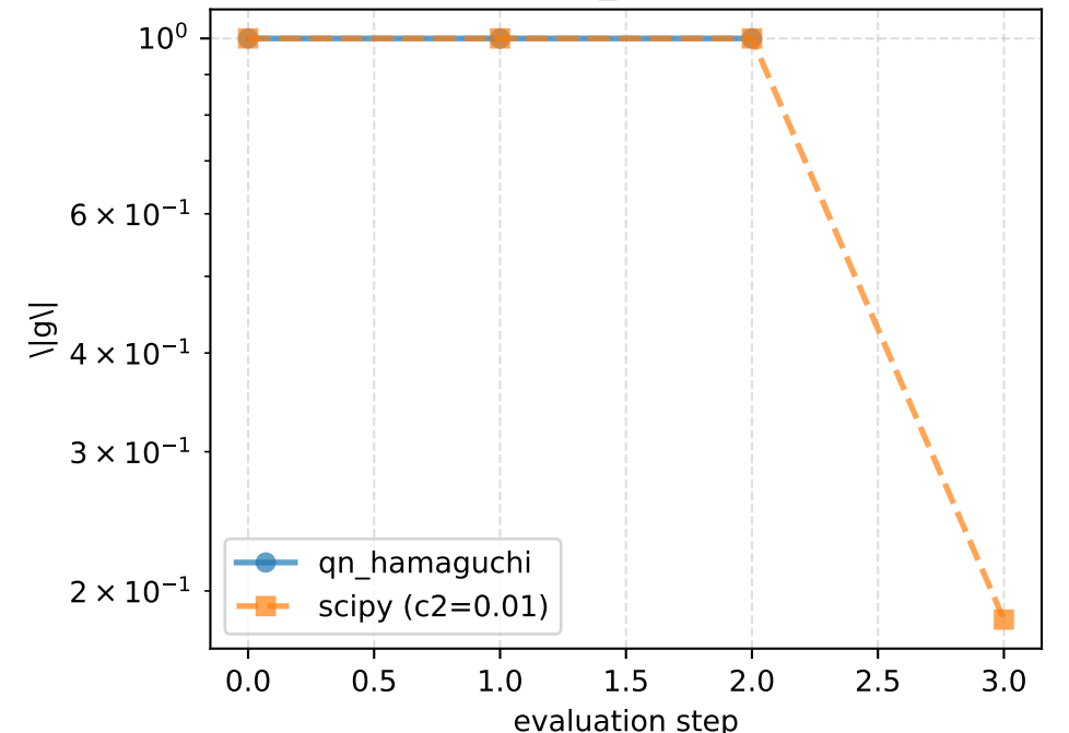
ConvexEvenPolynomial_4 - Gradient norm history
