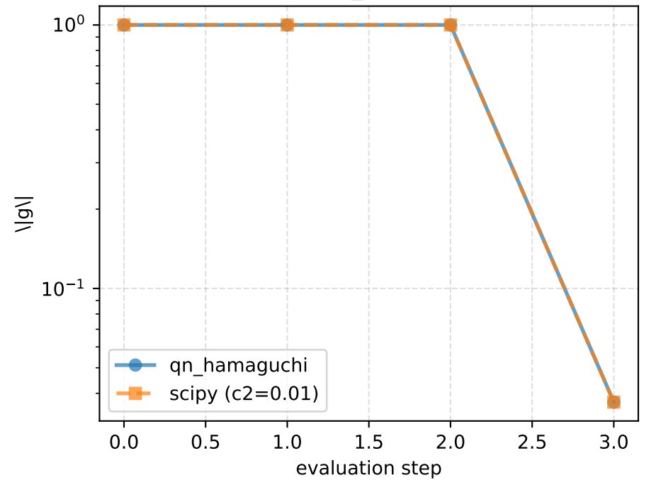
ConvexEvenPolynomial_4 - Gradient norm history
