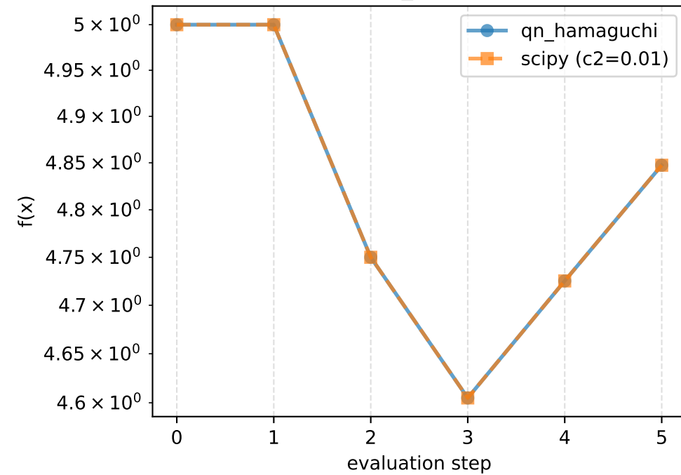
ConvexEvenPolynomial_4 - Function value history
