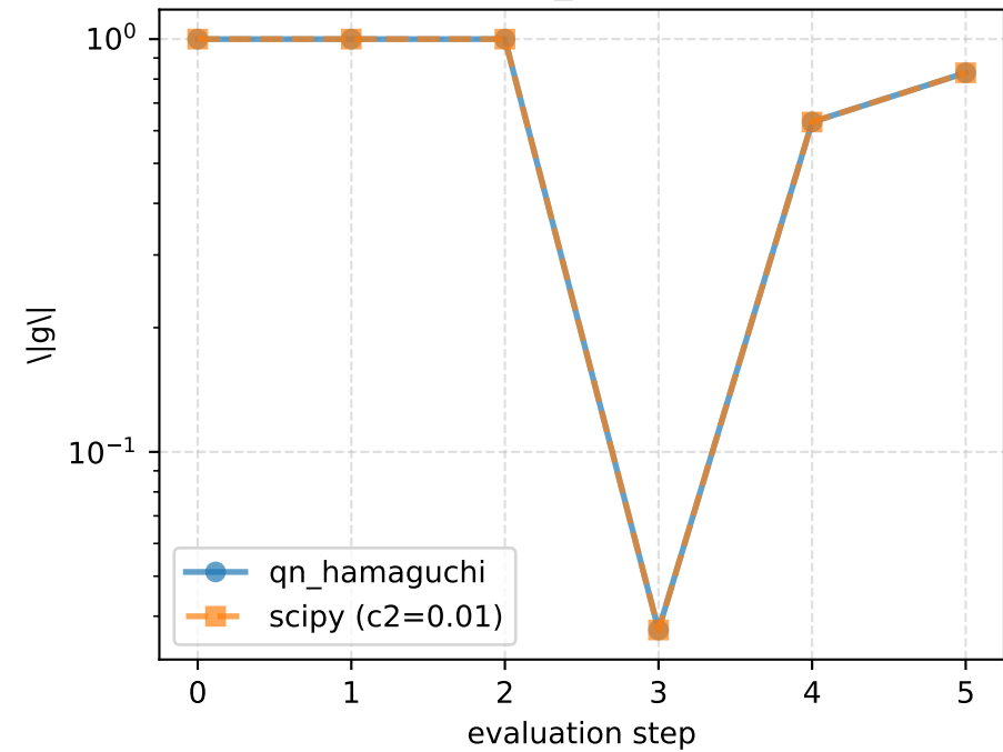
ConvexEvenPolynomial_4 - Gradient norm history
