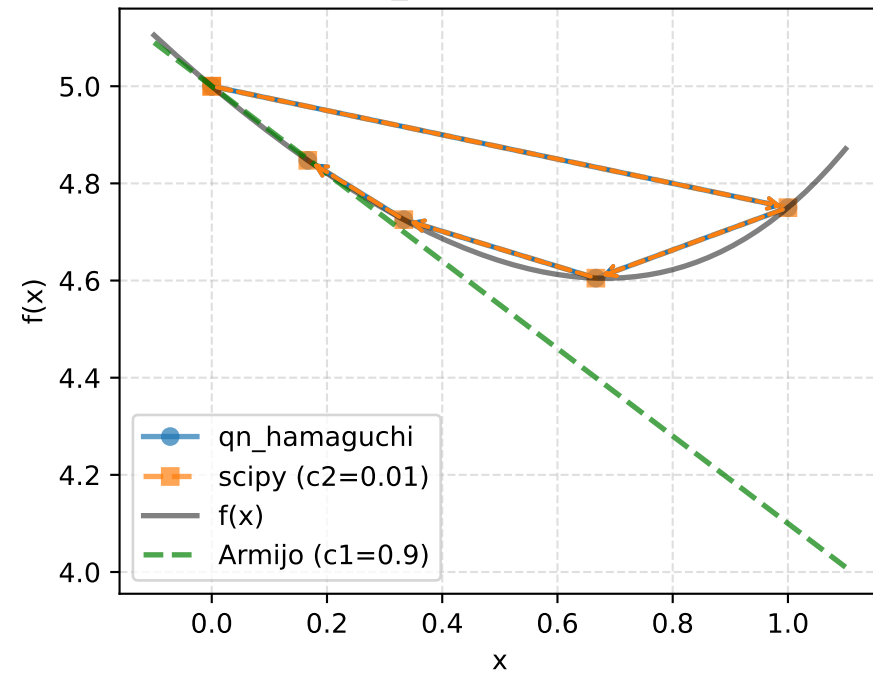
ConvexEvenPolynomial_4 - Function value and search paths
