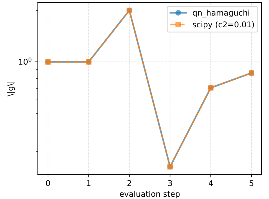
ConvexEvenPolynomial_6 - Gradient norm history
