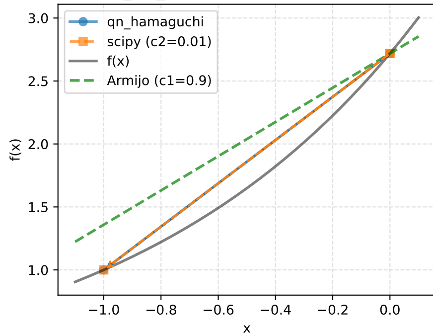
Exponential_1.0_0.0 - Function value and search paths
