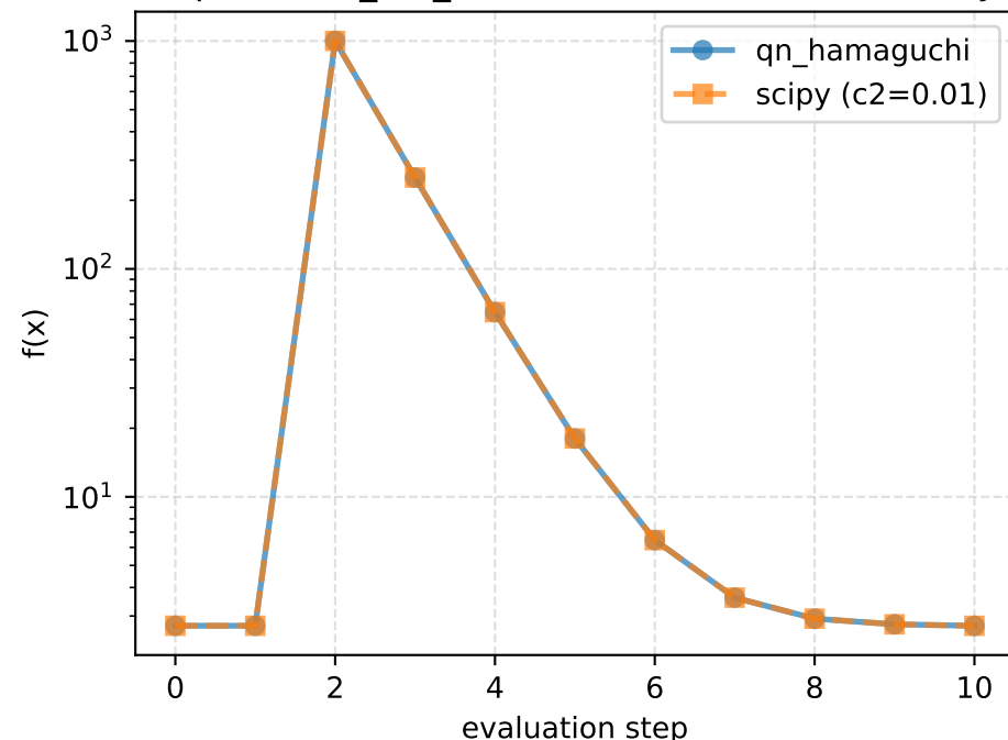
Exponential_1.0_1000.0 - Function value history
