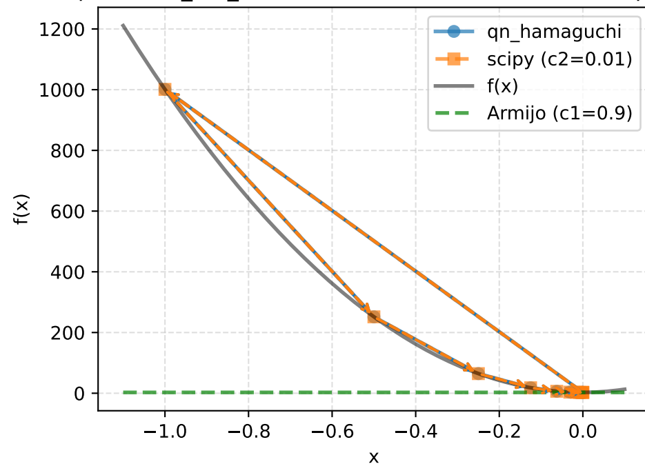
Exponential_1.0_1000.0 - Function value and search paths
