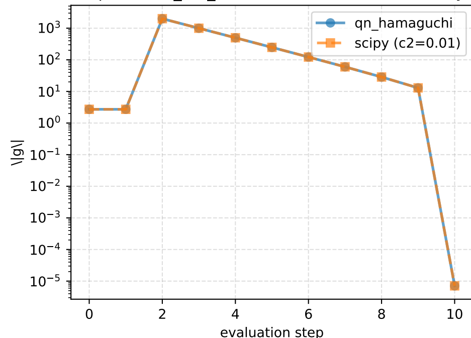
Exponential_1.0_1000.0 - Gradient norm history
