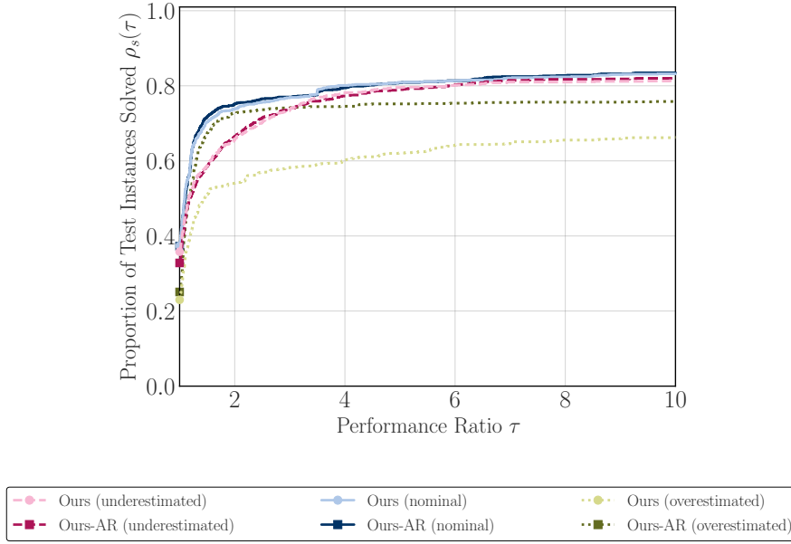
Fig. 3: Performance profiles for error-bound misspecification under function-value-only noise of level 10^{-3} and \epsilon_{\text{gtol}} = 10^{-2} .
