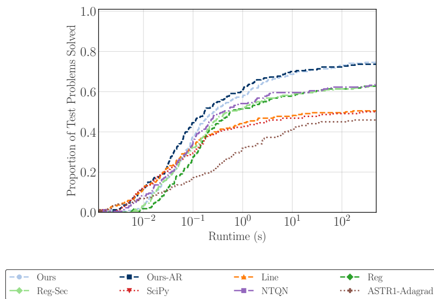
Fig. 5: Proportion of 32-bit test problems attaining \varepsilon_{\text{gtol}} = 10^{-3} as a function of runtime.
