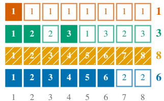
mt-spinwait
