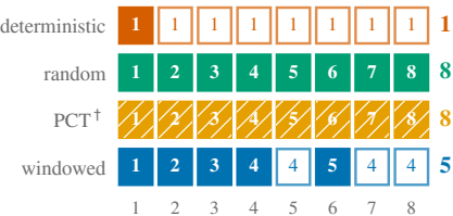
mt-crosscall
