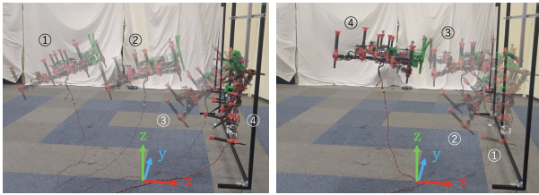
Fig.11: Perching experiment
