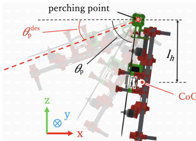
Fig.7: Takeoff control in pendulum-perching
