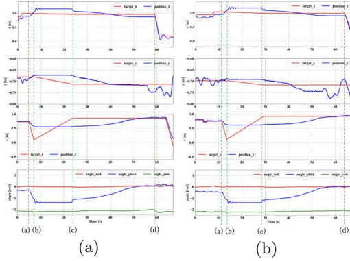
Fig.12: Plots of position and angle during perching
