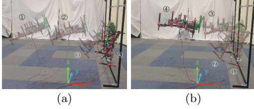
Fig.11: Perching experiment
