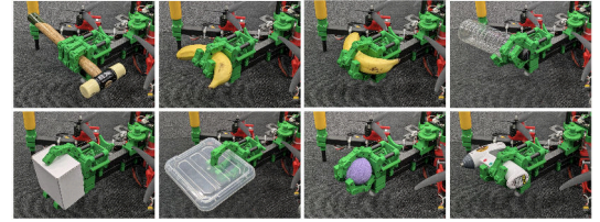
Fig.9: Grasping experiment with various shape objects
