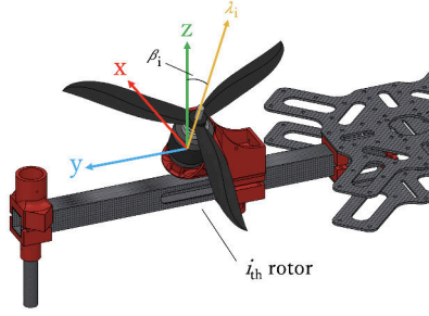
Fig.6: Coordinate arrangement on the base quadrotor
