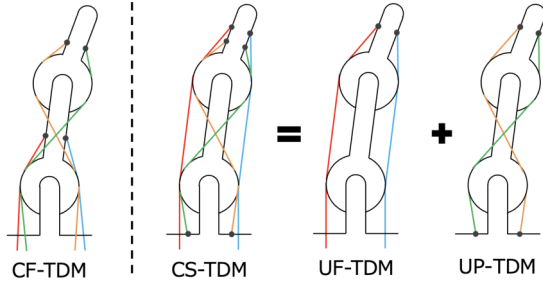
(a) Tendon-driven mechanisms
