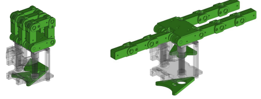
(b) Closed hand (c) Open hand Fig.3: Design of the Tri-force system and hand
