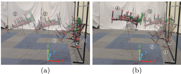
Fig.11: Perching experiment
