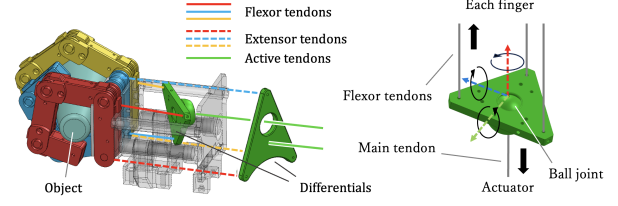
(a) Tri-force hand grasping slanted object
