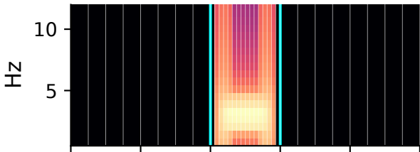
Foveated: 8 + 16 + 8 bins
