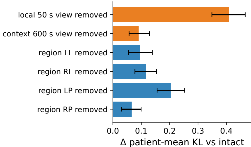
Deletion on the full test (P, seed 101)
