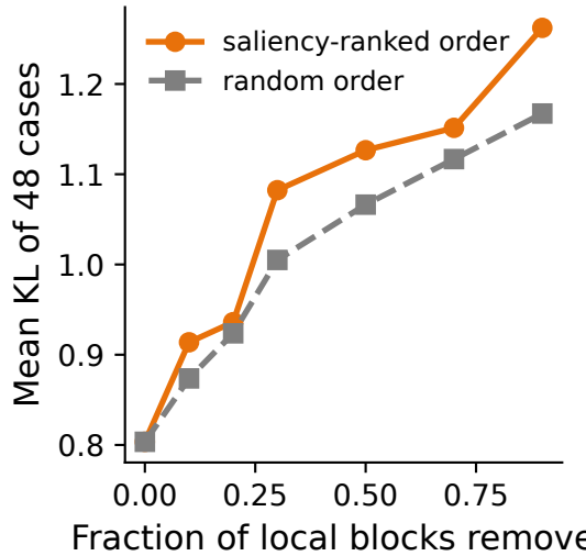
Ranked vs random deletion
