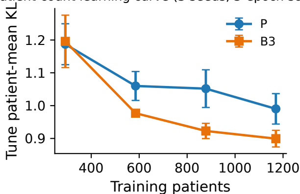
Patient-count learning curve (3 seeds, 3-epoch schedule)
