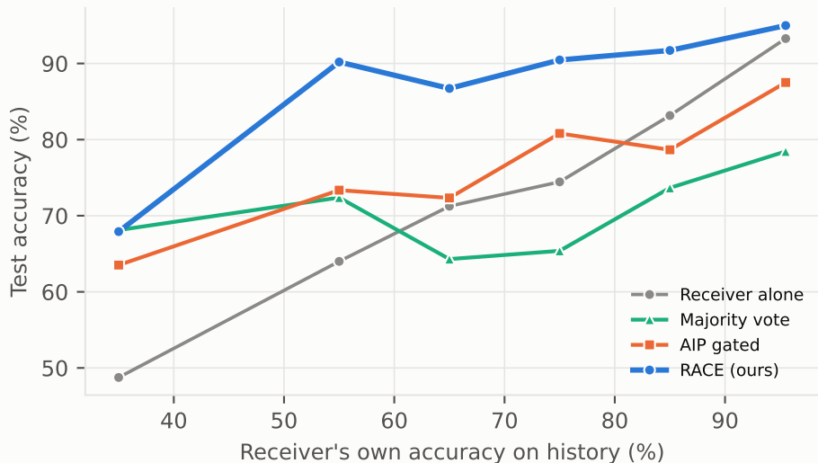
Mean accuracy by receiver competence
