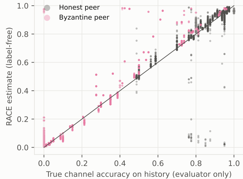
Channel estimation: r = 0.977 , MAE = 0.032
