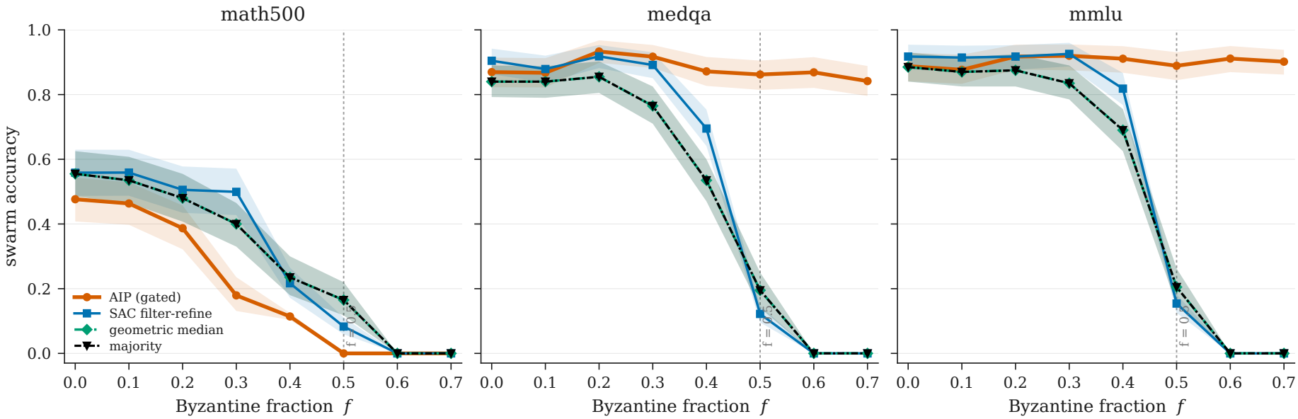
Accuracy vs Byzantine fraction — mix_all4, complete graph, p_{obs} = 1 , coherent adversary
