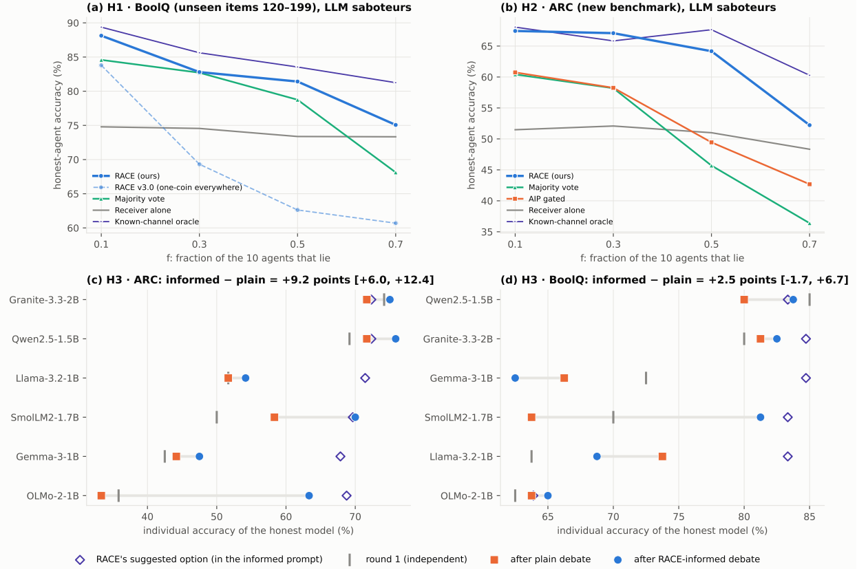
Figure 15: E10 (pre-registered). (a) H1: BoolQ items never shown to the live models; v3.1 (solid) against v3.0 (dashed), majority vote, the receiver alone and the known-channel oracle. (b) H2: ARC, a benchmark new to the live swarm. (c, d) H3: individual accuracy of each honest model in round 1 (bar), after a plain debate (square) and after a RACE-informed debate (dot); diamonds give the accuracy of the option the informed prompt suggested (after the warm-up). LLM saboteurs (solo, rushing, colluding), five seeds, TEST split.
