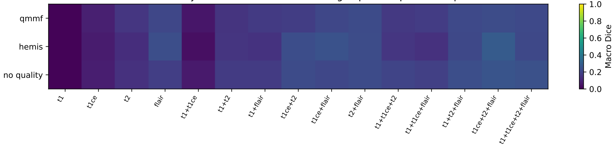
Macro Dice by available modalities: fixed 8-group development sample
