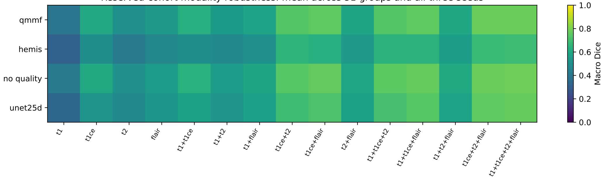
Reserved-cohort modality robustness: mean across 51 groups and all three seeds
