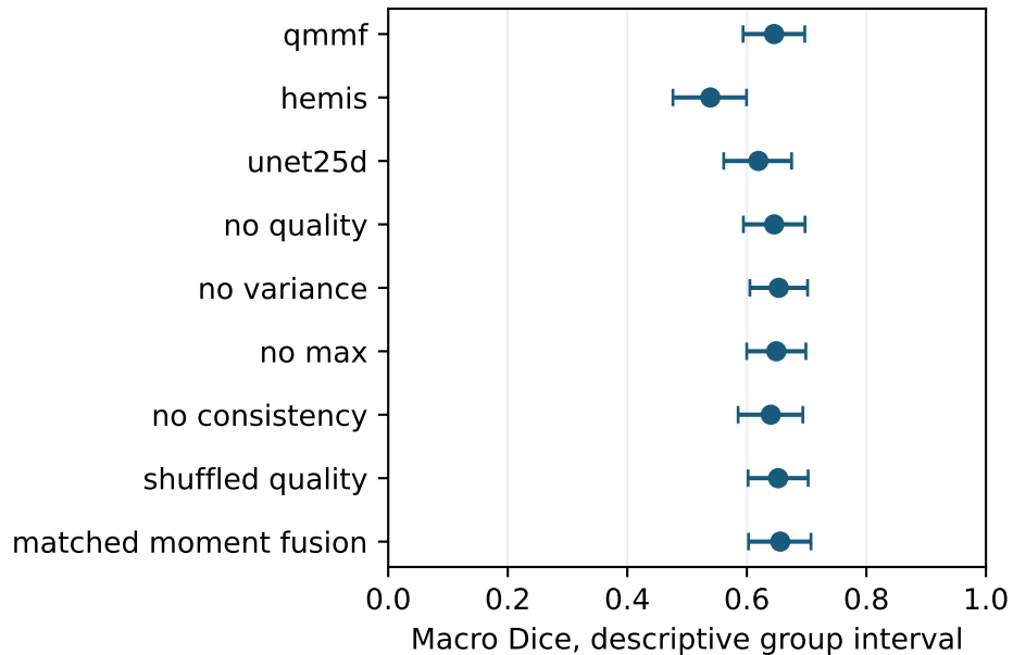
15-subset mean, 16 development groups
