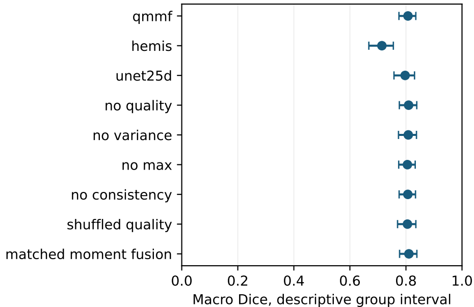
Full modalities, outer development fold
