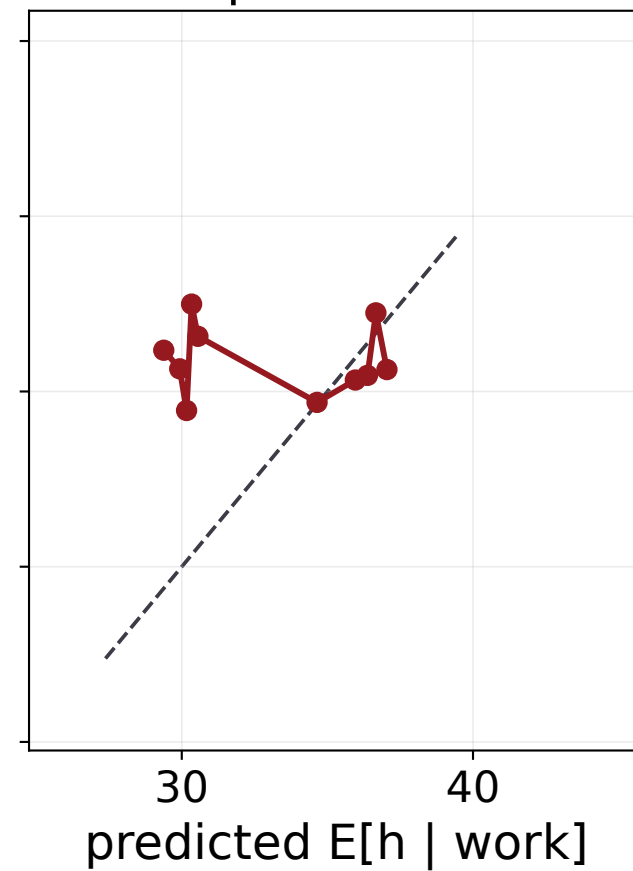
coupled women
