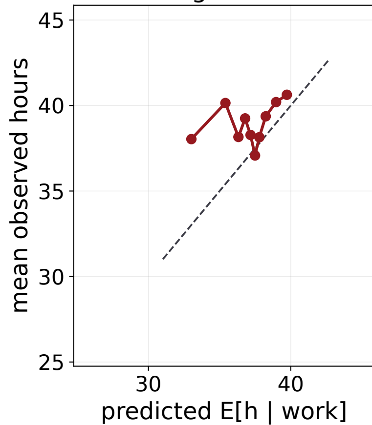
single men
