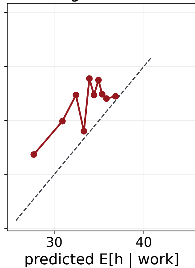
single women
