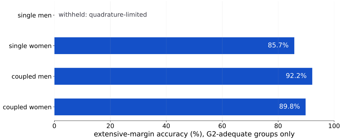
Figure 7: Weighted extensive-margin accuracy against the model’s own simulated 95 per cent band (500 outcome vectors at the fitted estimates), for the three groups that clear the pre-registered numerical-adequacy gate; single men do not clear it and are withheld. Source: POSFIT v3 (MNL_posfit, branch diagnostics/posfit-v3, commit 96693269), same extensive-margin numbers as v2b, reframed against the simulated band.
