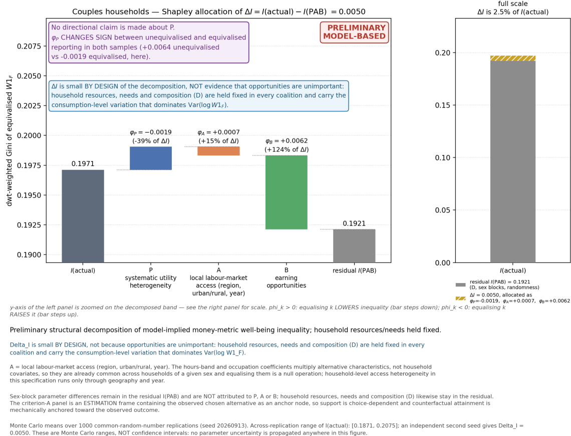
Figure 10: Couple estimation sample: coalition Gini levels and the exact Shapley allocation of \Delta I across P, A and B, with the sign instability of P annotated. Modified-OECD-equivalised W_F^1 ; Monte Carlo ranges over 1,000 replications, not confidence intervals. Preliminary, model-based.
