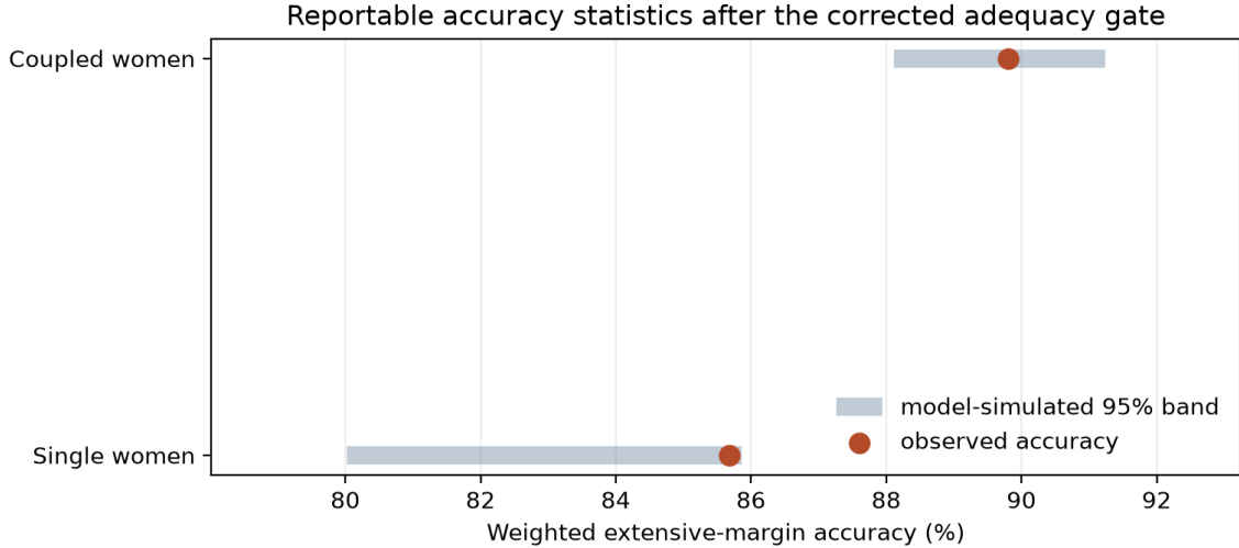
Figure 7: Corrected weighted extensive accuracy. Only single women and coupled women clear the preregistered numerical-adequacy gate. The statistics for single men and coupled men are quadrature-limited and withheld. Source: POSFIT v3b.
