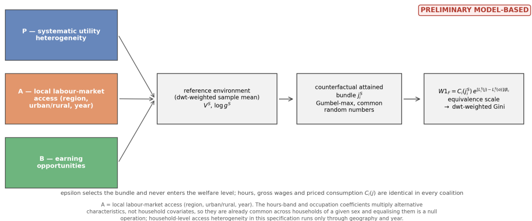
Figure 11: The eight P/A/B counterfactual coalitions, built from the accepted model by equalising household-constant covariates within a block. Node-level alternative characteristics are preserved in every coalition; only household-constant covariates are equalised. Preliminary, model-based.
