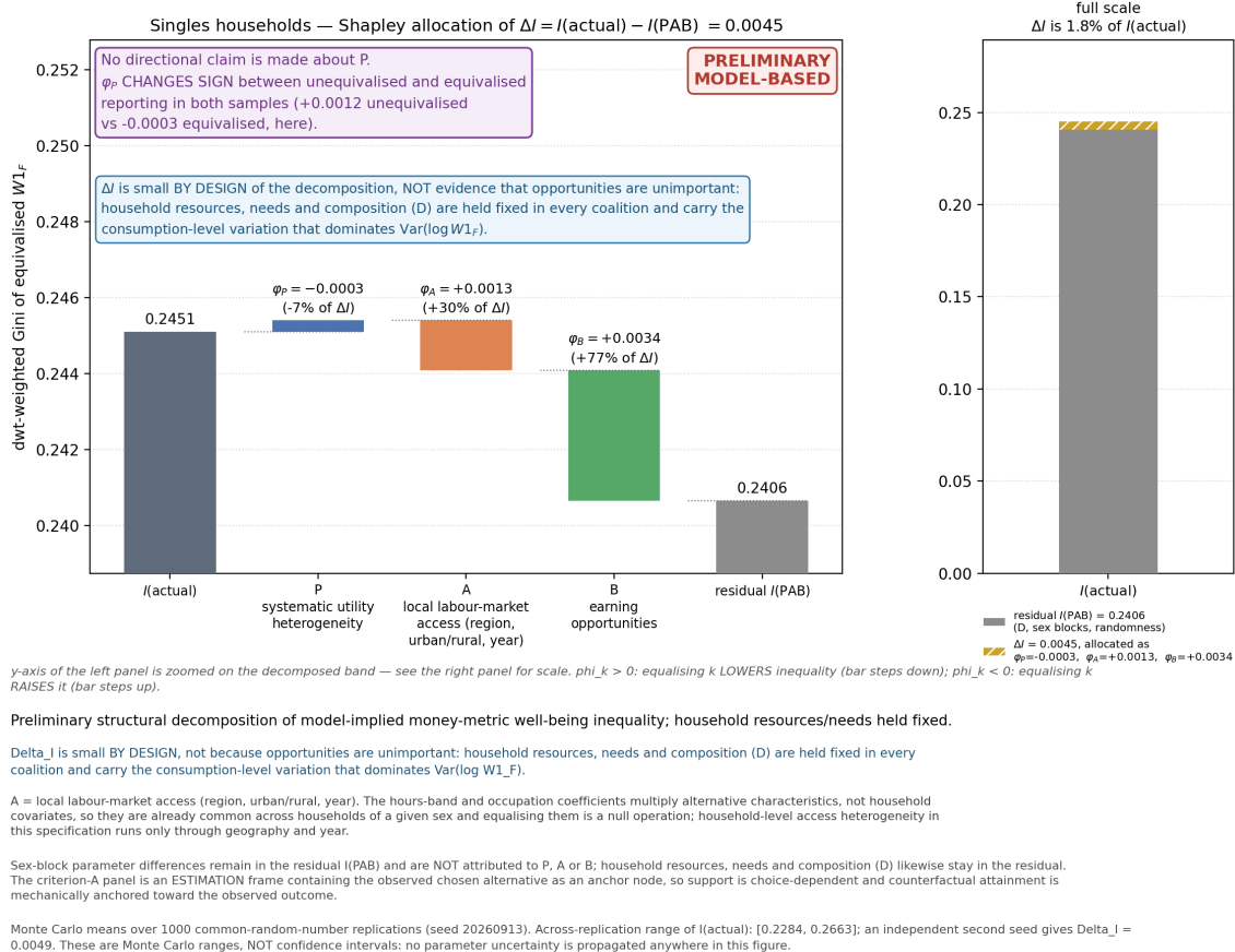
Figure 12: Single-adult estimation sample: coalition Gini levels and the exact Shapley allocation of \Delta I across P, A and B, with the sign instability of P annotated. Modified-OECD-equivalised W_F^1 ; Monte Carlo ranges over 1,000 replications, not confidence intervals. Preliminary, model-based.
