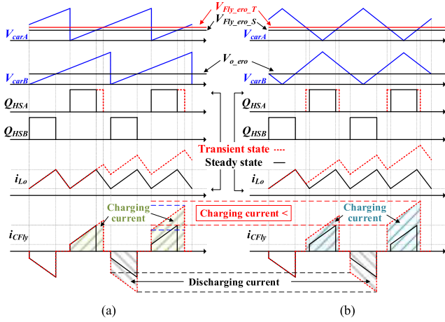
FIGURE 10. Differences in C_{Fly} charging and discharging currents according to the carrier signal during control operation (in the case of V_{Fly} < V_{in}/2 , M < 0.5 ): (a) sawtooth wave carrier signal, (b) triangular wave carrier signal.
