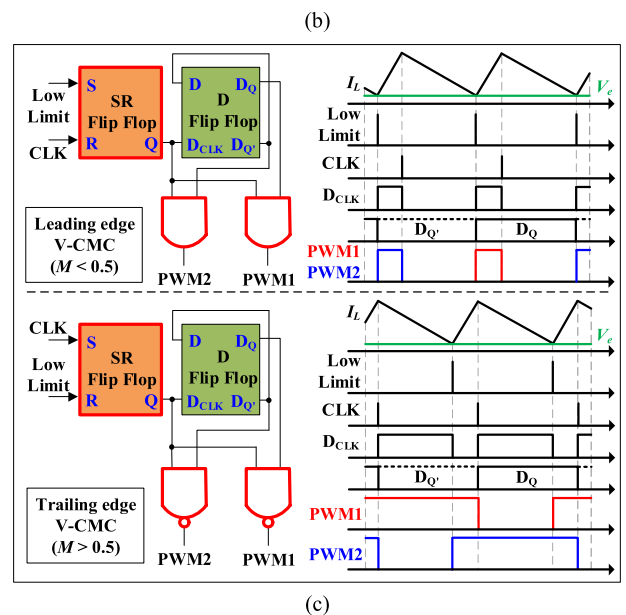
FIGURE 8. Block diagram of conventional CMC method: (a) 3-level buck converter circuit diagram with CMC method applied, (b) block diagram of P-CMC, and (c) block diagram of V-CMC.
