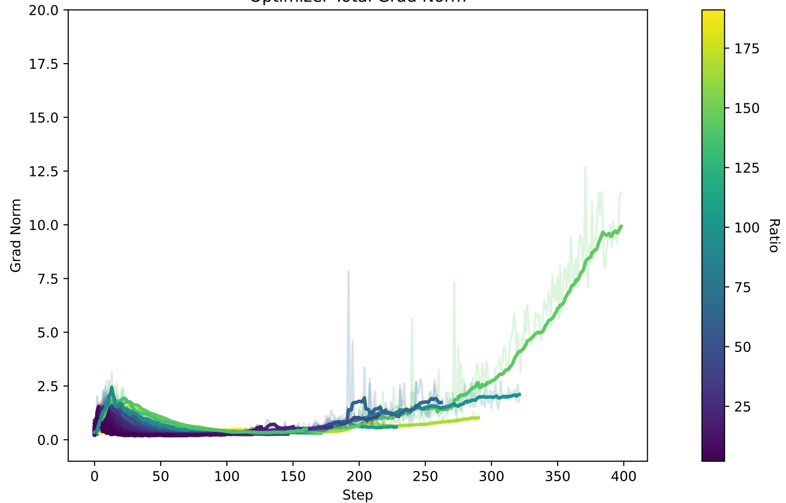
Optimizer Total Grad Norm
