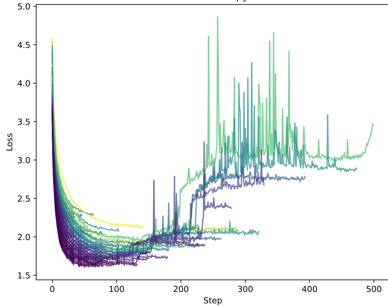
Train CrossEntropyLoss
