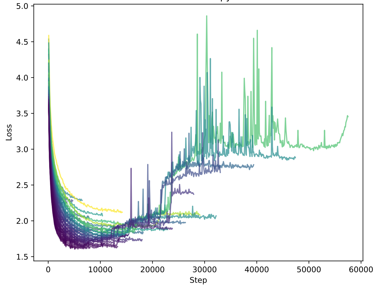
Train CrossEntropyLoss
