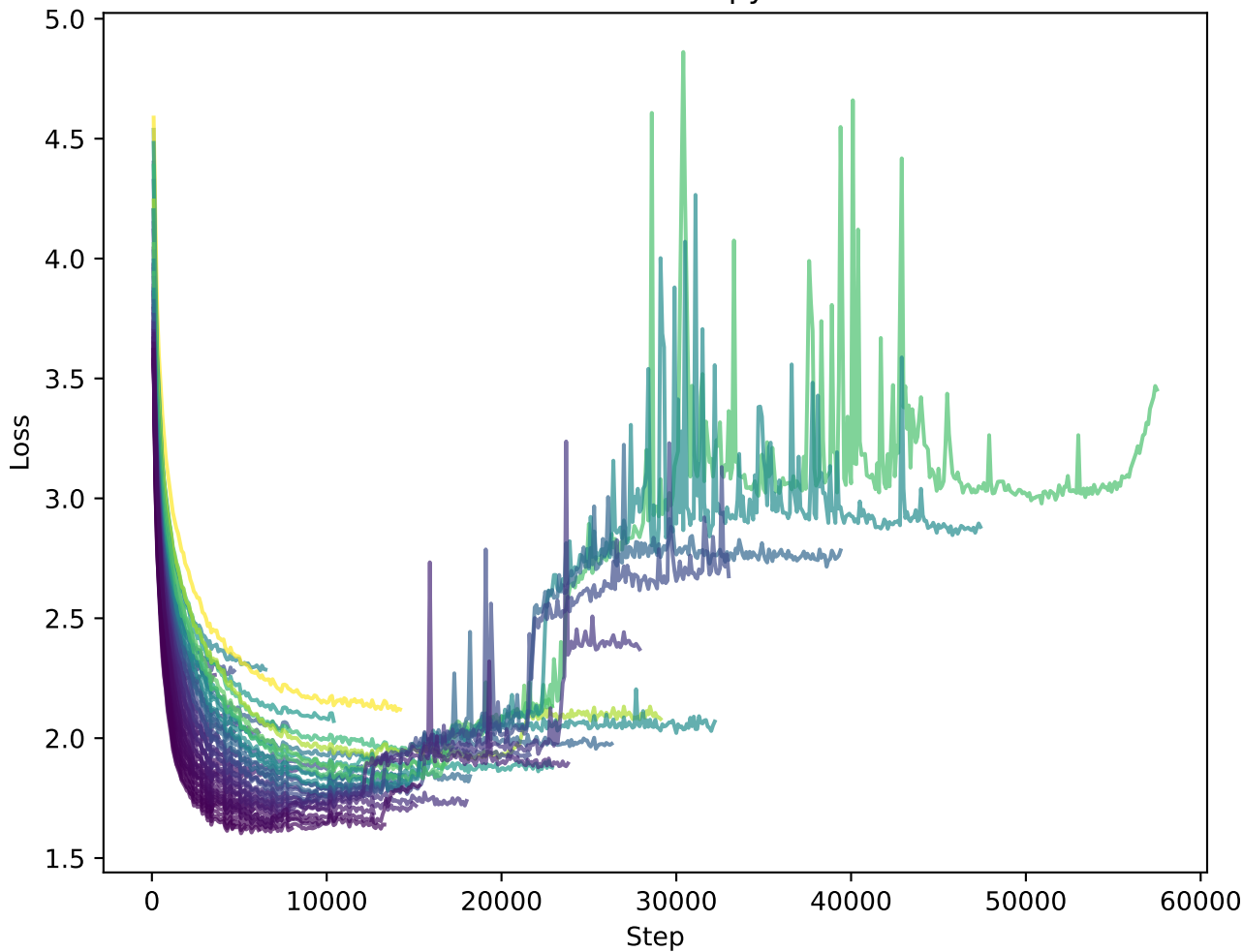
Train CrossEntropyLoss
