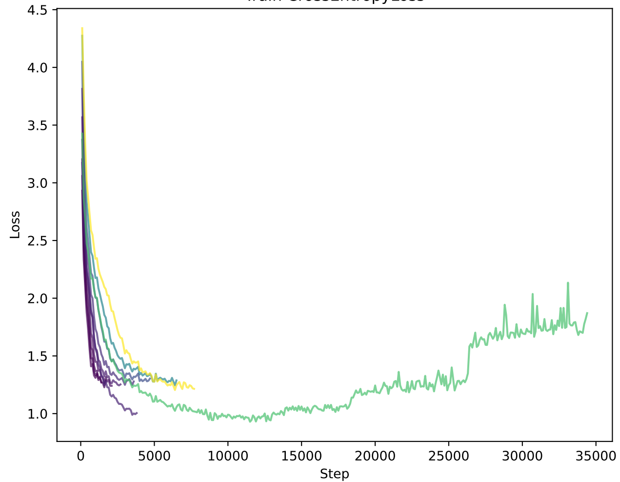
Train CrossEntropyLoss
