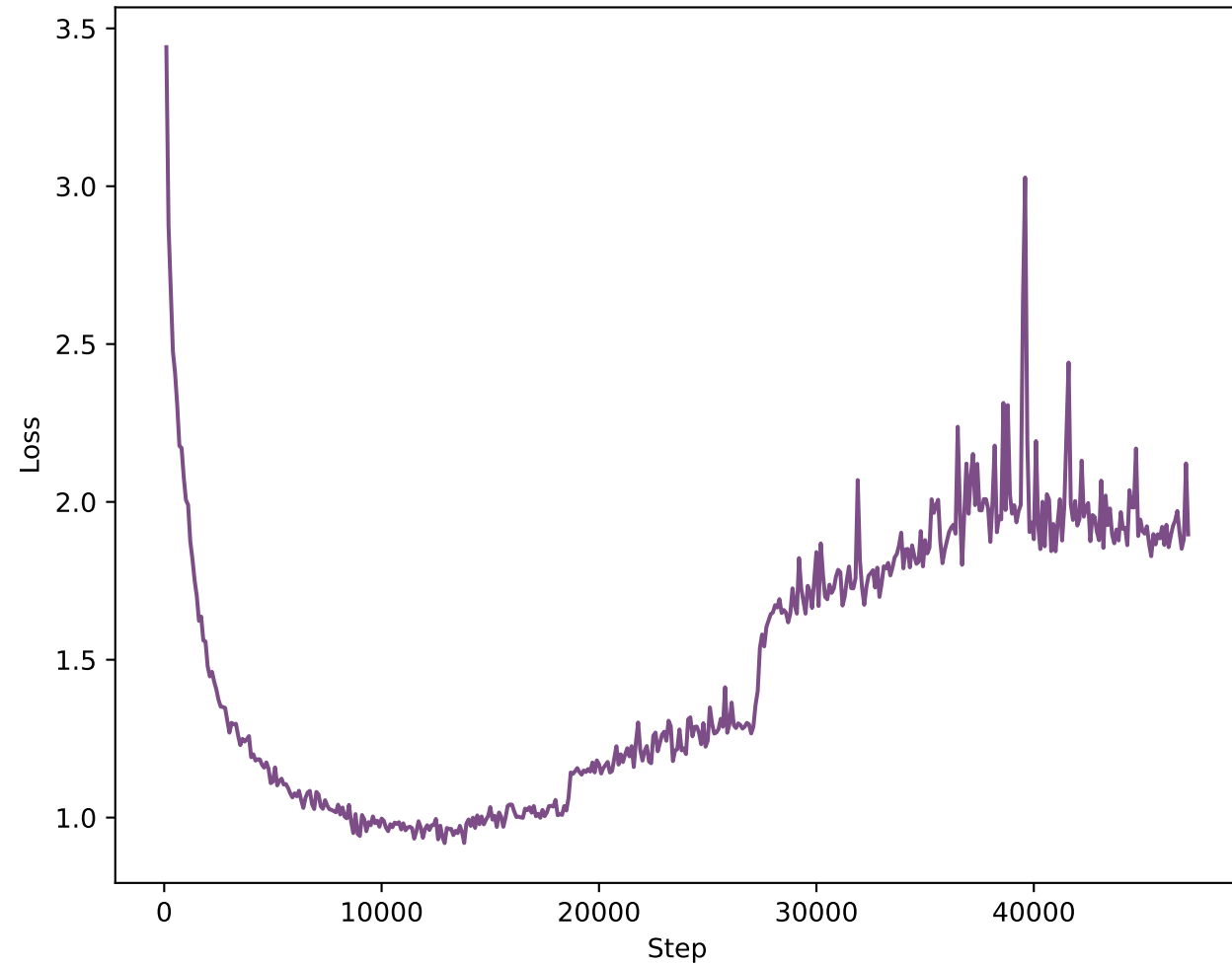
Train CrossEntropyLoss
