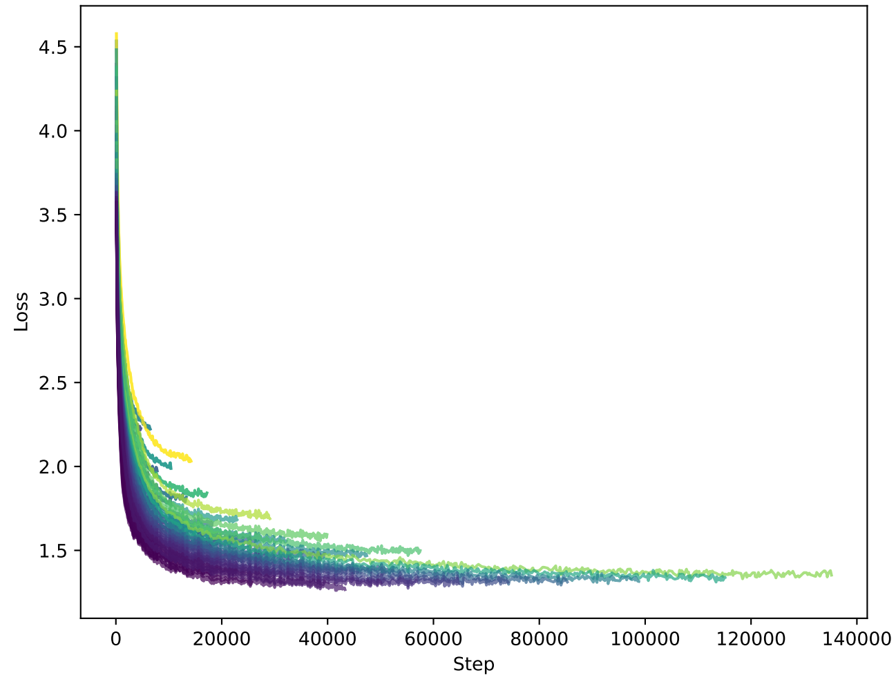
Train CrossEntropyLoss
