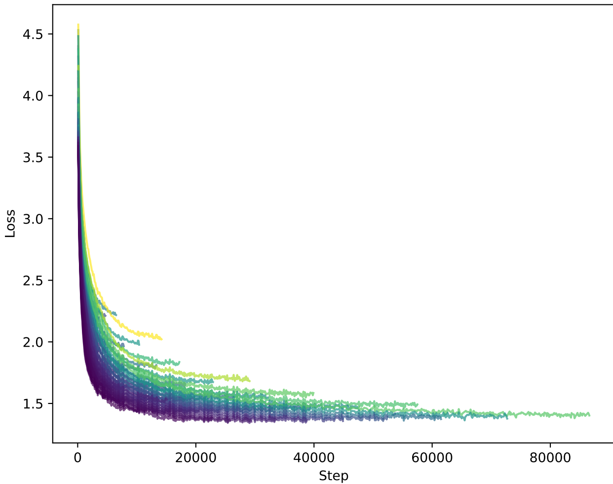
Train CrossEntropyLoss
