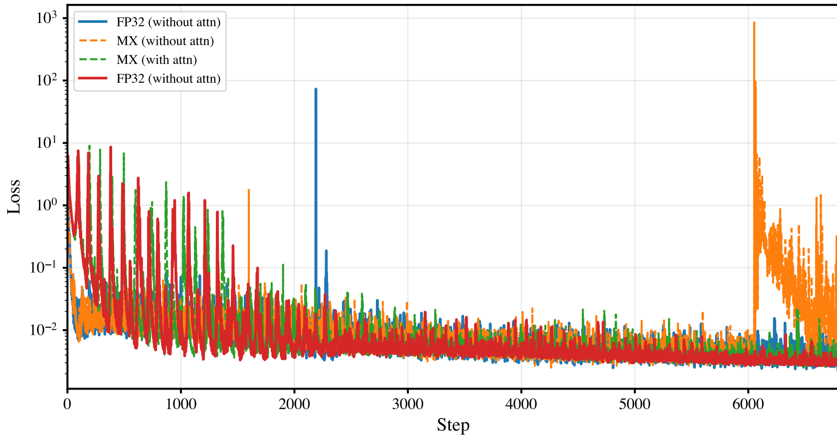
FP32 vs MX Loss (with/without attention)
