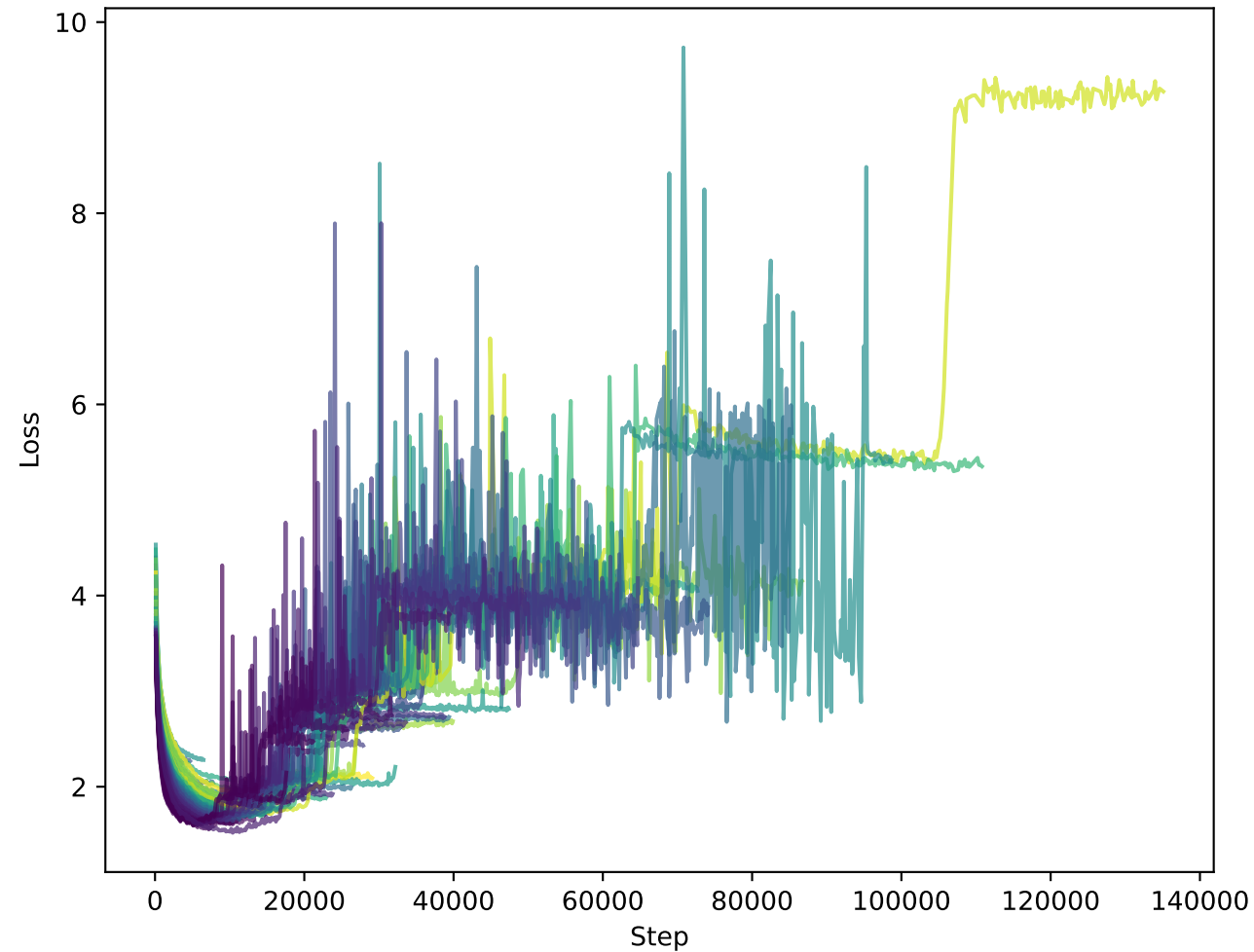
Train CrossEntropyLoss
