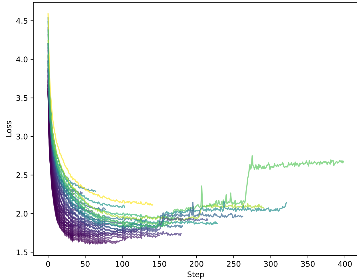
Train CrossEntropyLoss
