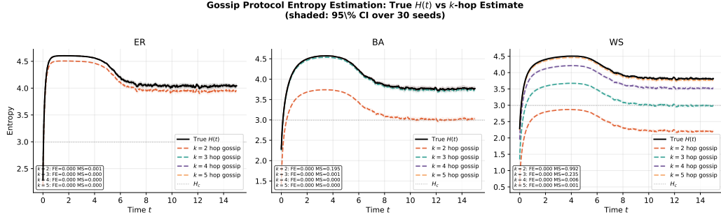
Figure 7: Gossip protocol entropy estimation: true H(t) (black) vs k = 2 (orange) and k = 3 (teal) hop estimates across three topologies ( n = 100 , N = 30 seeds). Annotations give false-early (FE) and missed-trigger (MS) rates.
