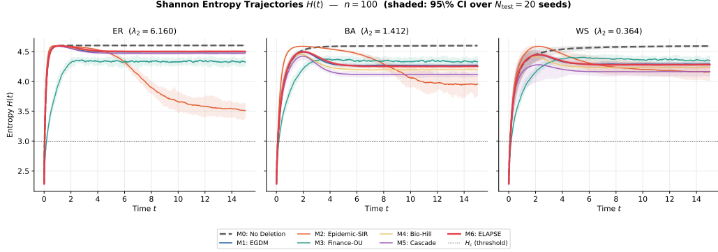
Figure 1: Mean Shannon entropy trajectories H(t) with 95% CI bands ( N_{\text{test}} = 20 seeds, n = 100 ). Each panel shows a topology; the dashed horizontal line marks H_c = 0.65H_{\max} . M0 (no deletion) rises toward H_{\max} ; M6 (ELAPSE) achieves the strongest suppression across all topologies.
