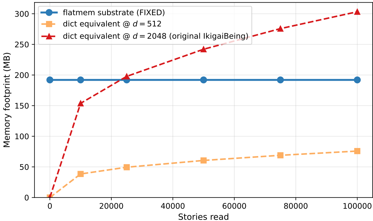
Substrate is flat; dict grows with vocabulary
