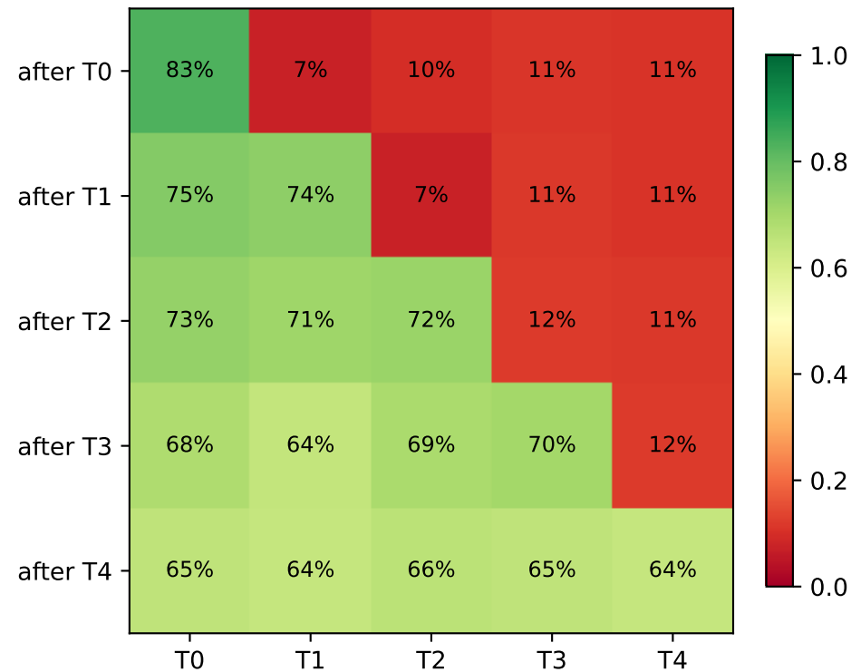
flatmem final avg 65% BWT -10%
