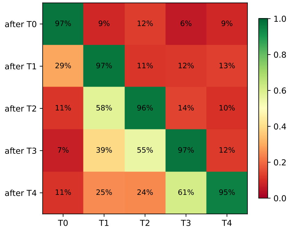
sklearn-mlp final avg 43% BWT -67%
